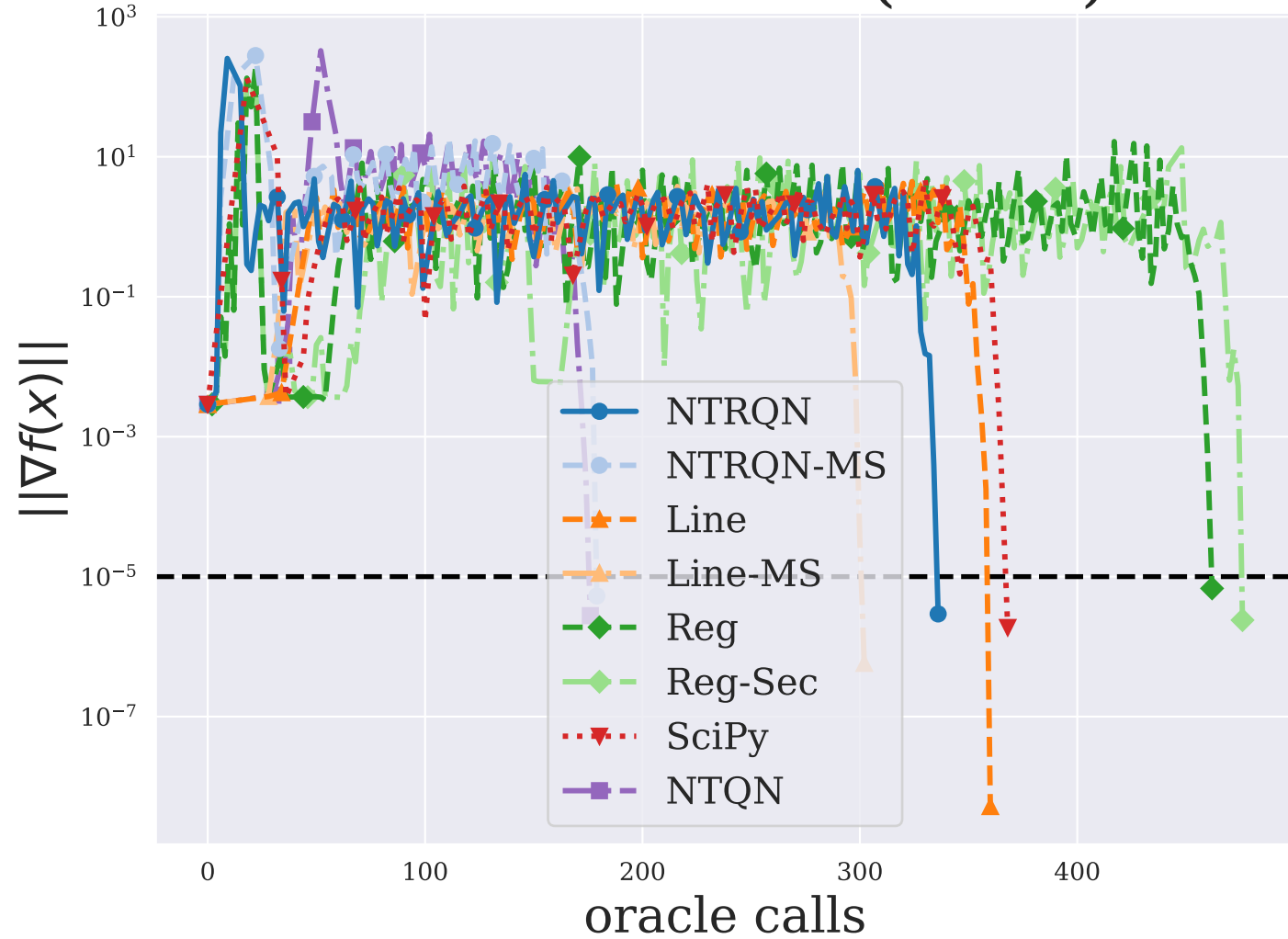
ROSENBRTU ( n = 2 )
