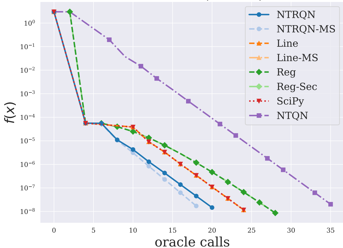
SISSER ( n = 2 )
