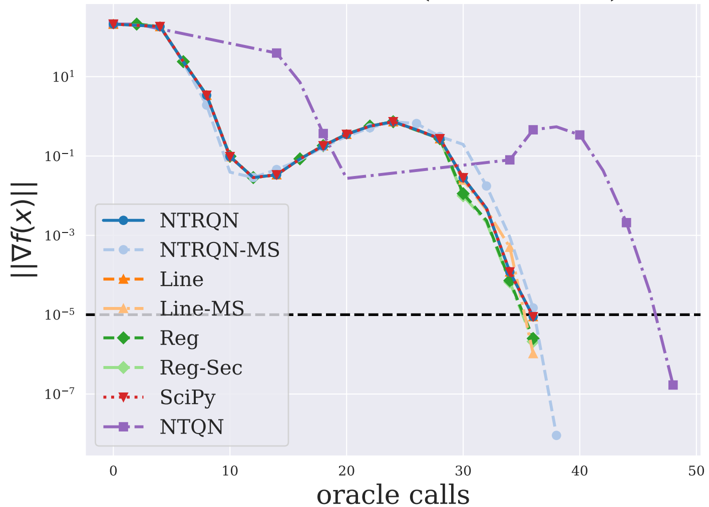
SROSENBR ( n = 5000 )
