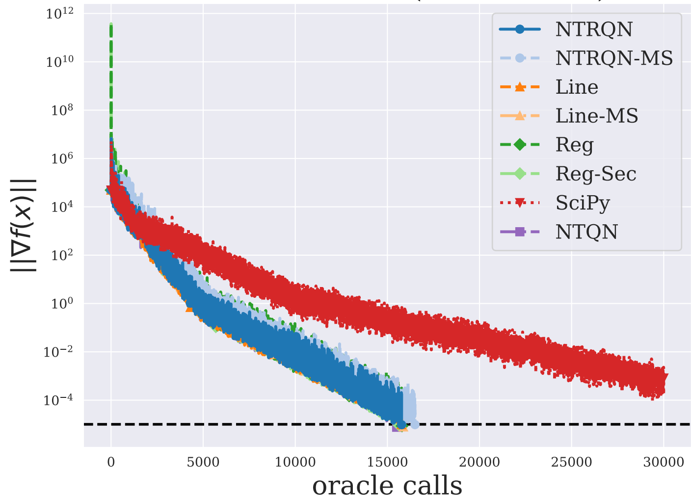
SSBRYBND ( n = 5000 )
