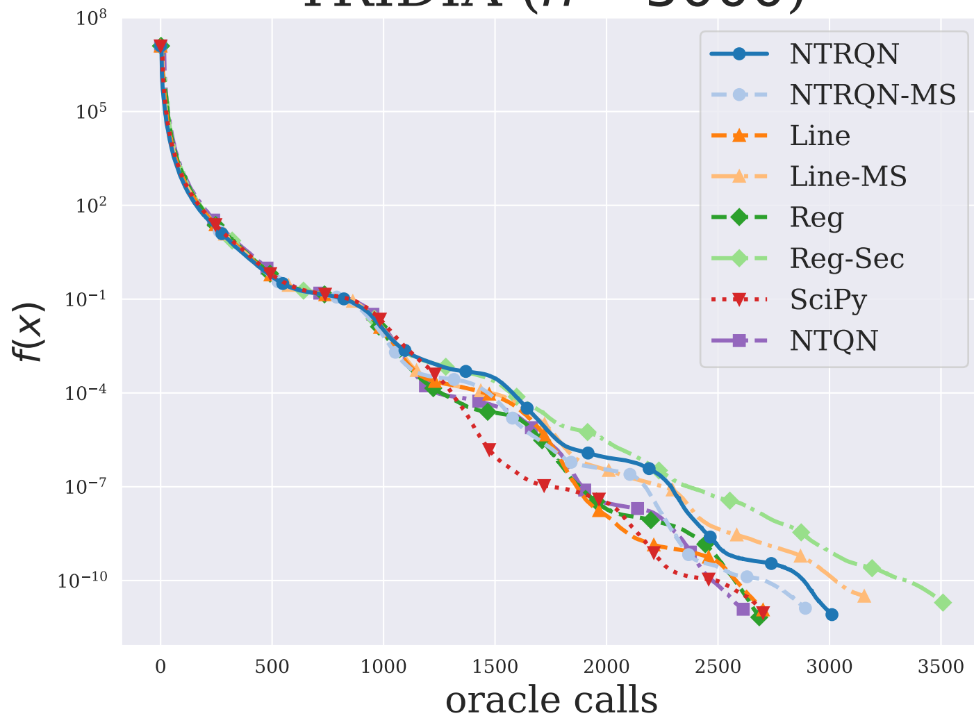
TRIDIA ( n = 5000 )
