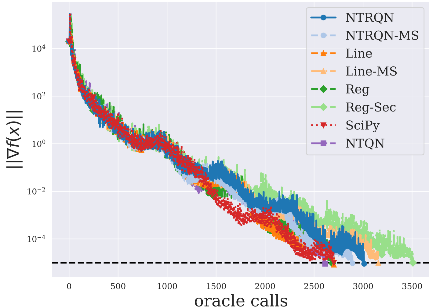
TRIDIA ( n = 5000 )
