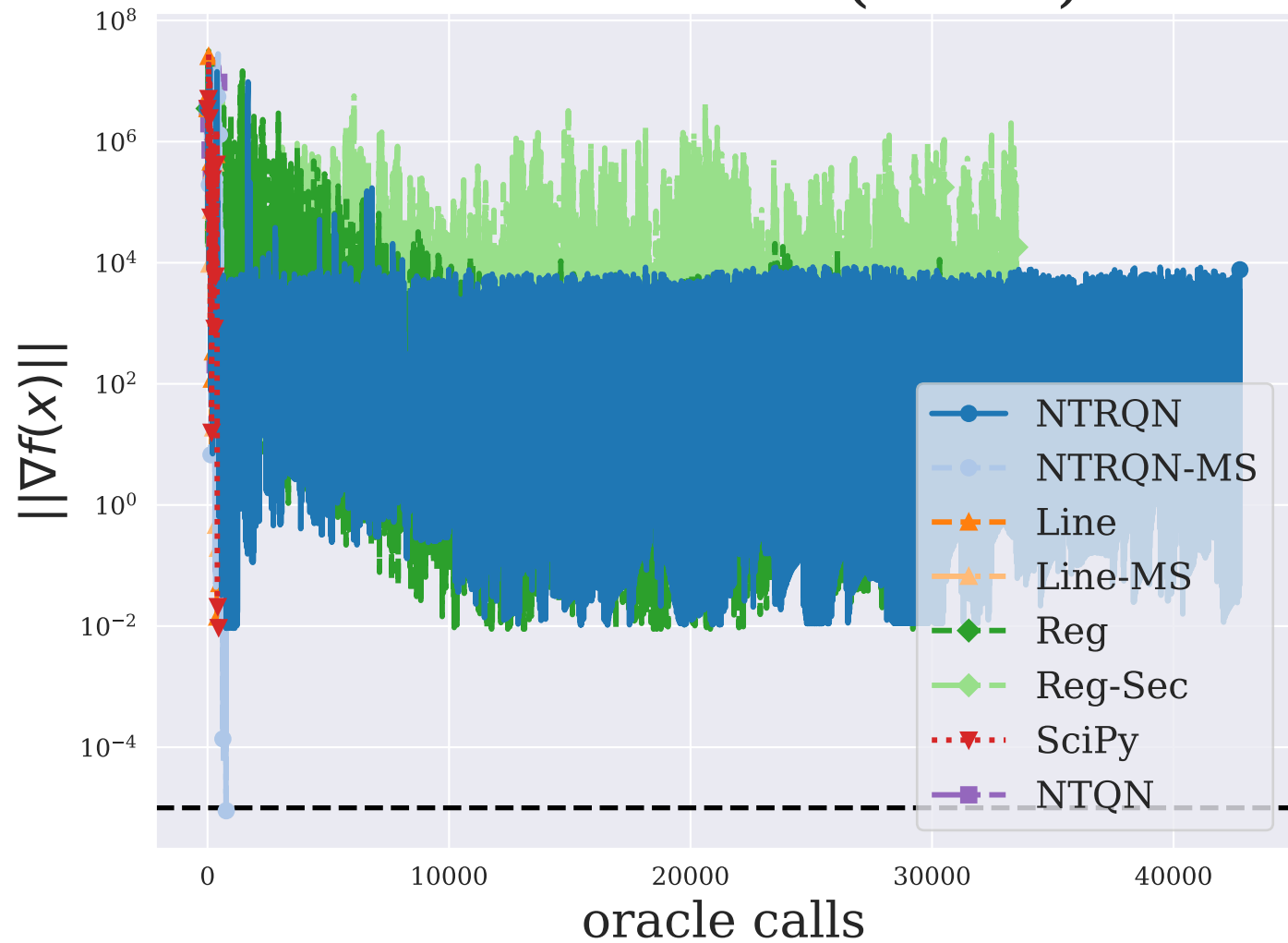
VESUVIALS ( n = 8 )
