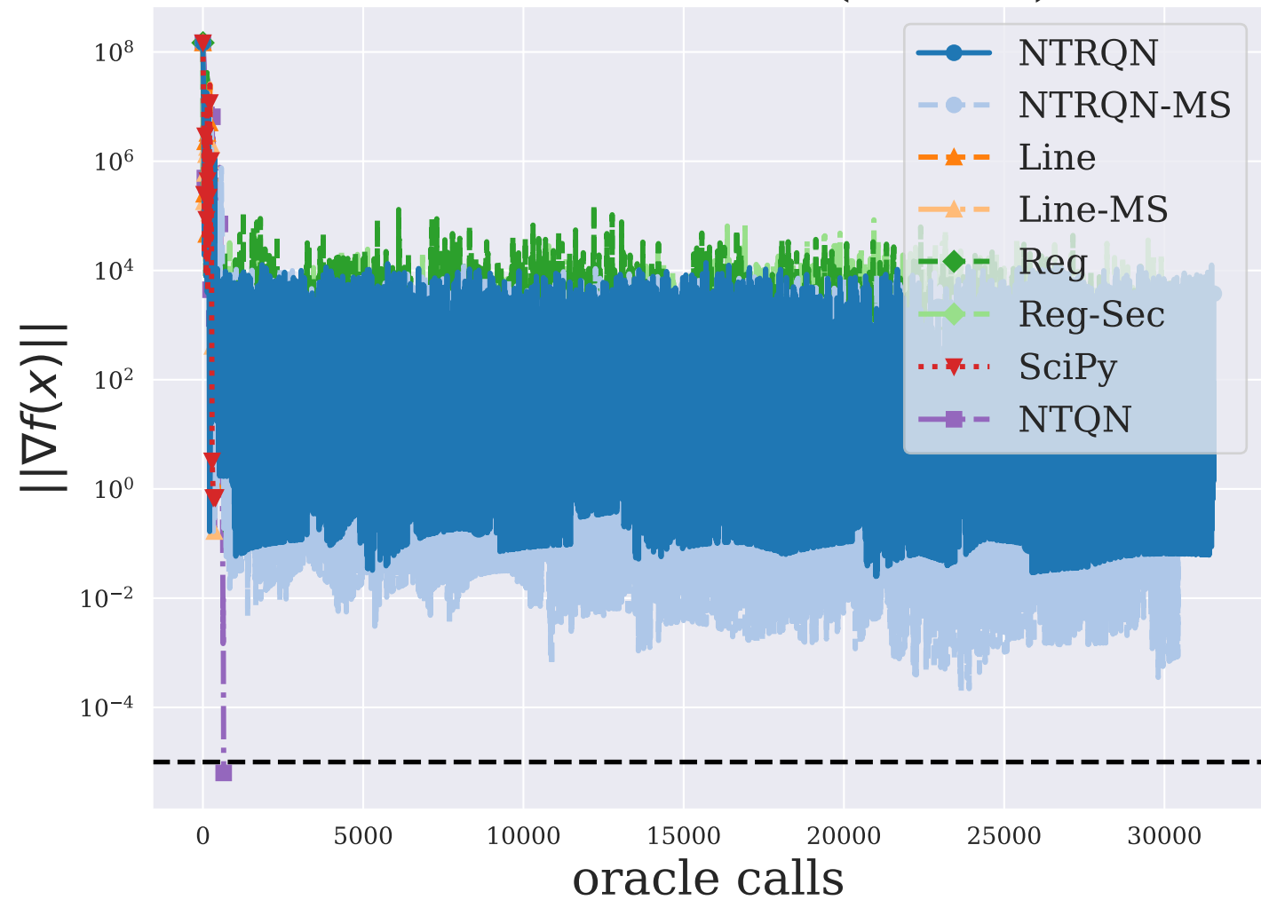
VESUVIOLS ( n = 8 )
