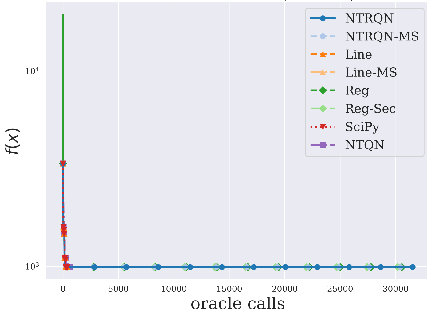
VESUVIOLS ( n = 8 )
