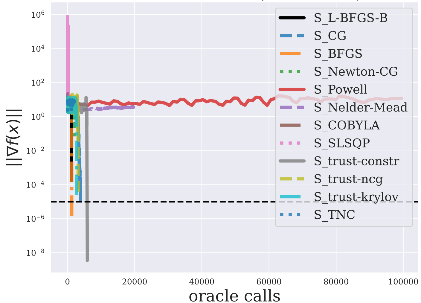
Rosenbrock ( n = 100 )
