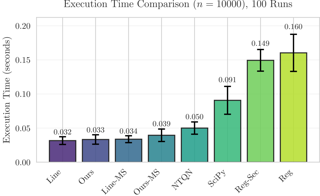
Figure 3: Mean execution times for the experiment in section 6.3. This plot roughly indicates the extra computational overhead of each method. Error bars represent one standard deviation over 100 runs.
