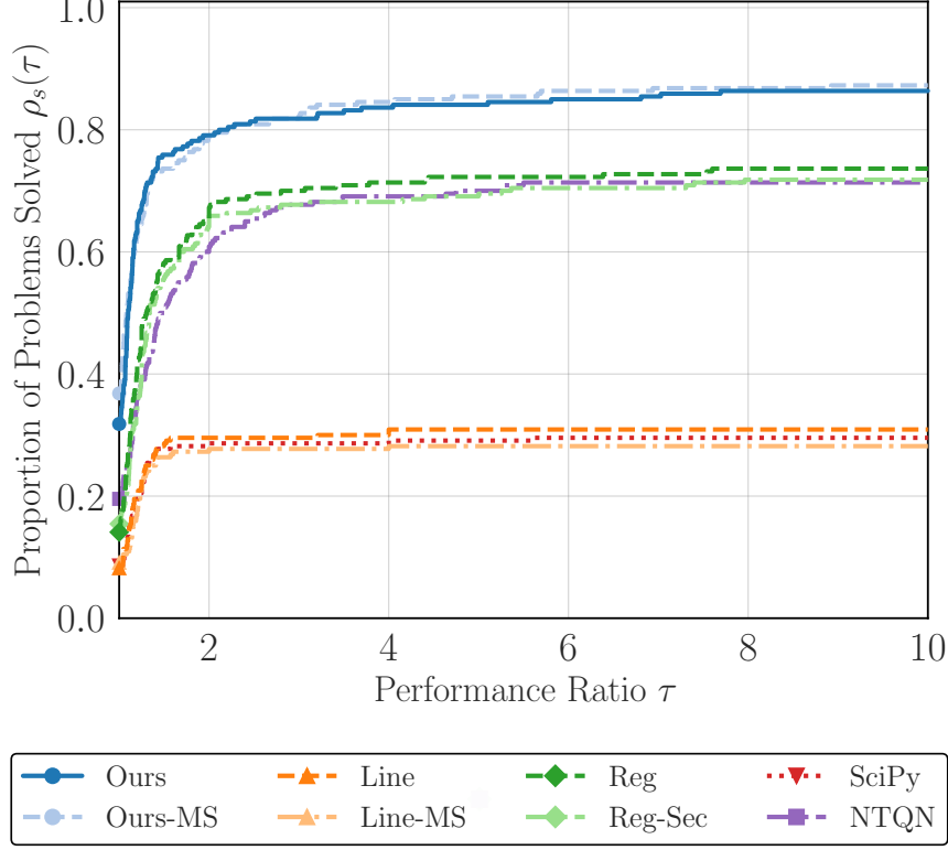
Figure 1: Performance profile for artificial noise setting (level of 10^{-3} ) and \epsilon_{\text{gtol}} = 10^{-2} .
