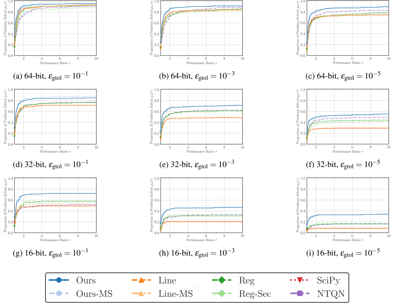
Figure 2: Performance profiles across different floating-point precisions (64-, 32-, and 16-bit) and tolerance levels. The results demonstrate the robustness of the proposed methods.
