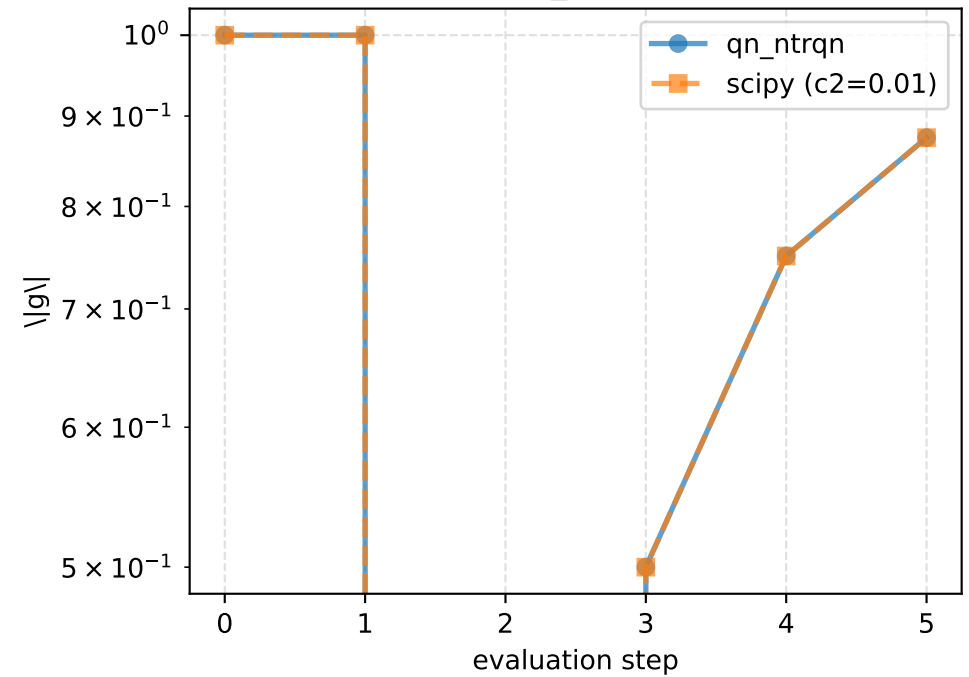
ConvexEvenPolynomial_2 - Gradient norm history
