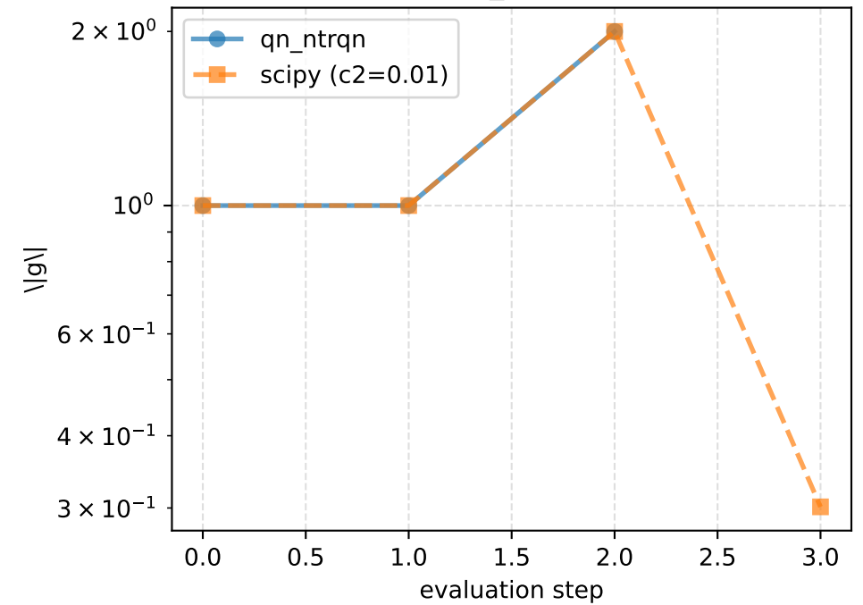
ConvexEvenPolynomial_6 - Gradient norm history
