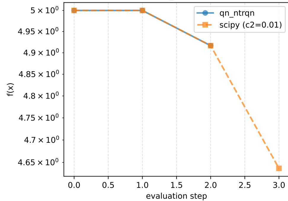
ConvexEvenPolynomial_6 - Function value history
