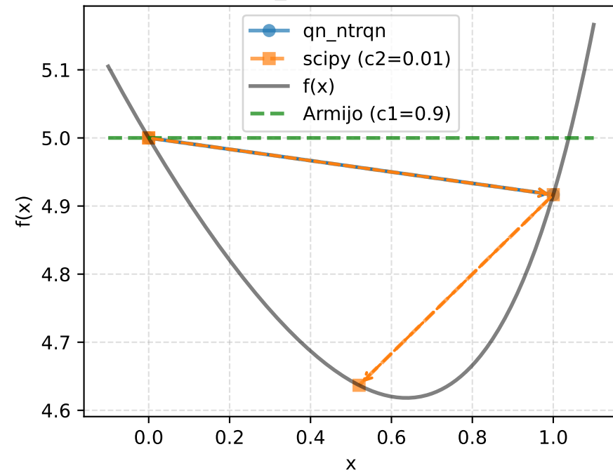
ConvexEvenPolynomial_6 - Function value and search paths
