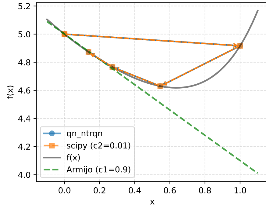
ConvexEvenPolynomial_6 - Function value and search paths
