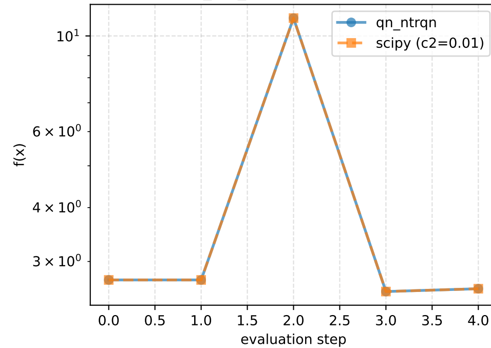
Exponential_1.0_10.0 - Function value history
