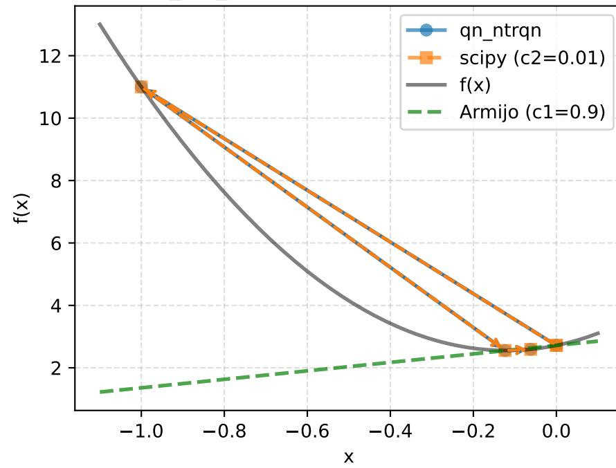
Exponential_1.0_10.0 - Function value and search paths
