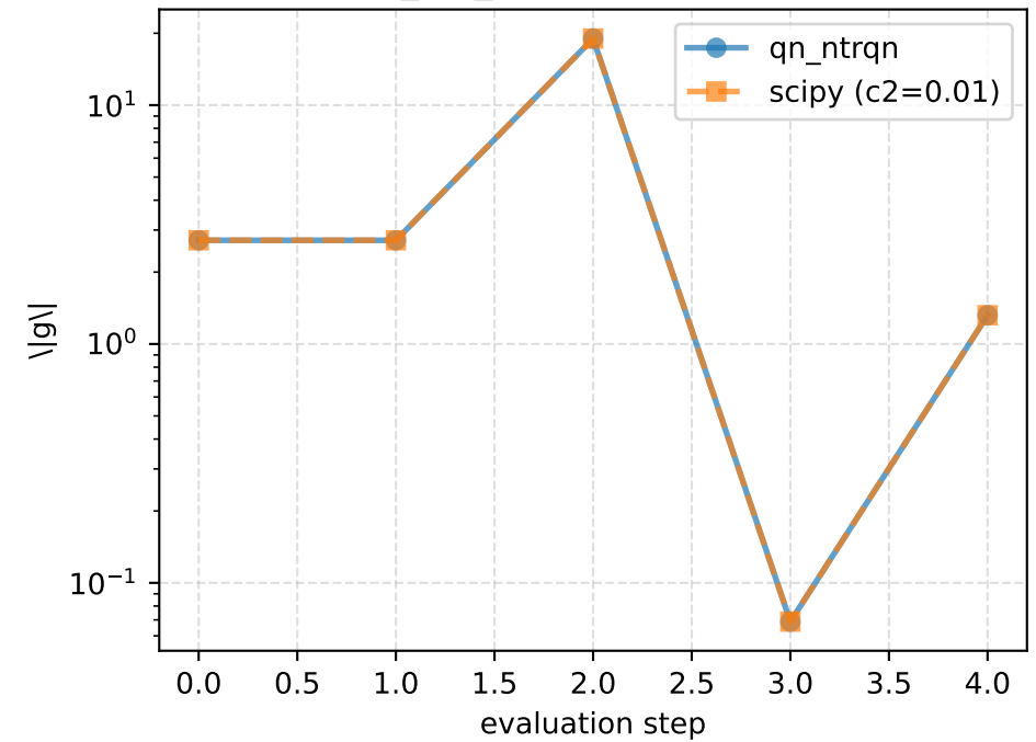
Exponential_1.0_10.0 - Gradient norm history
