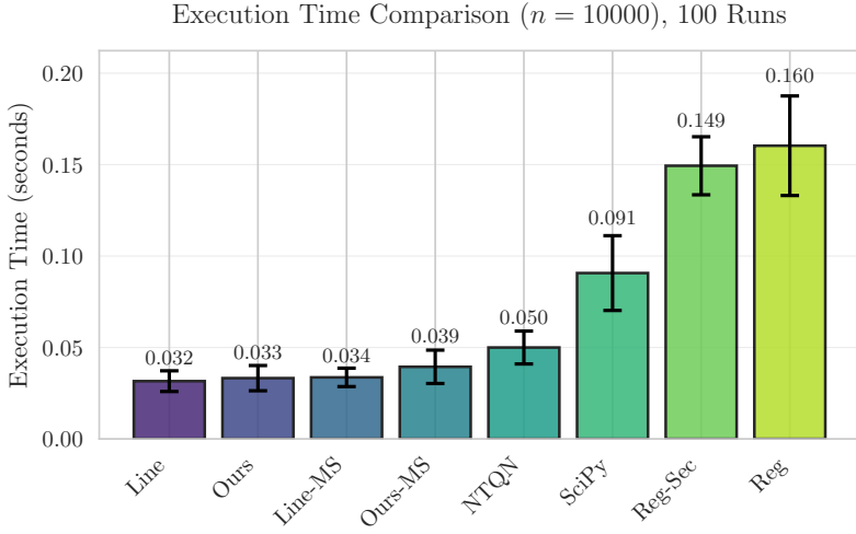
Fig. 3: Mean execution times for the experiment in ???. This plot roughly indicates the extra computational overhead of each method. Error bars represent one standard deviation over 100 runs.
