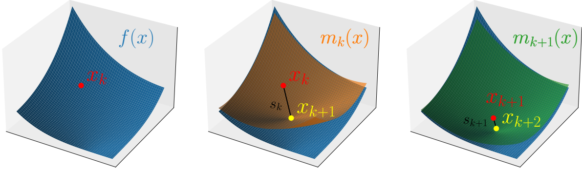
Figure 10: Conceptual illustration of quasi-Newton methods. (1) Given the objective function f (blue surface) and the current point x_k (red point). (2) Move to the minimizer x_{k+1} (yellow cross) of the quadratic model m_k(x) (orange surface) constructed using the current approximate Hessian. (3) Update the quadratic model (green surface) and repeat this procedure.
