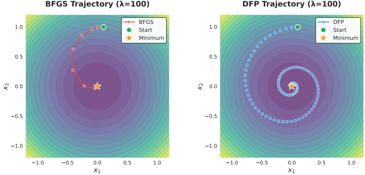
Figure 1: Iterative trajectories for BFGS and DFP methods when \lambda_1 = 100 . BFGS converges in 10 iterations while DFP requires 107 iterations, showing BFGS’s superior efficiency for large eigenvalue errors.
