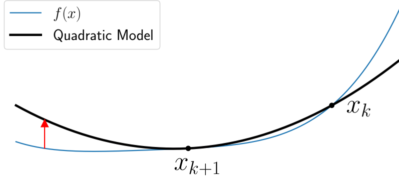
Figure 15: Function-value-matching modified secant equation. The function values f(x_k) and m_k^F(x_k) are matched at the previous point x_k .
