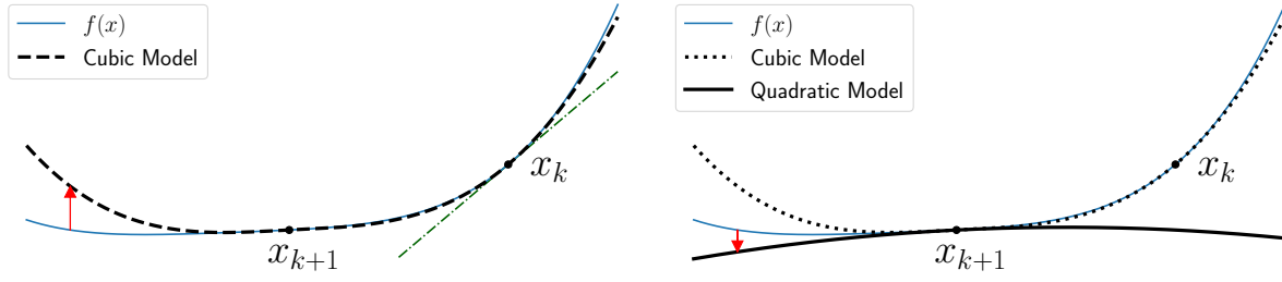
Figure 4: Cubic-augmented modified secant equation. The cubic term is incorporated into the model to simultaneously match both function value and gradient at the previous point. The model is constructed using the expansion up to the quadratic term.
