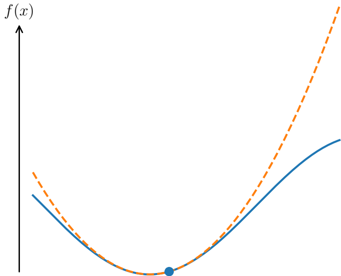
L -smoothness of f
