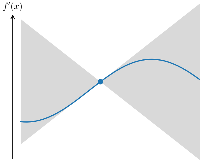
Lipschitz Continuity of \nabla f
