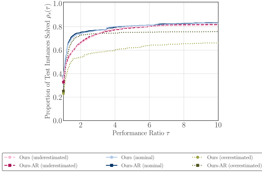
Fig. 3: Performance profiles for error-bound misspecification under function-value noise of level 10^{-3} , with \epsilon_{\text{gtol}} = 10^{-2} .
