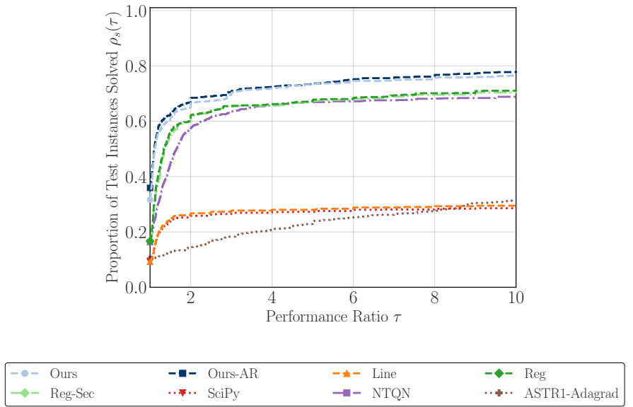
Fig. 1: Performance profiles under function-value noise of level 10^{-3} , with exact gradients, \epsilon_f = 10^{-2} , and \epsilon_{\text{gtol}} = 10^{-2} .
