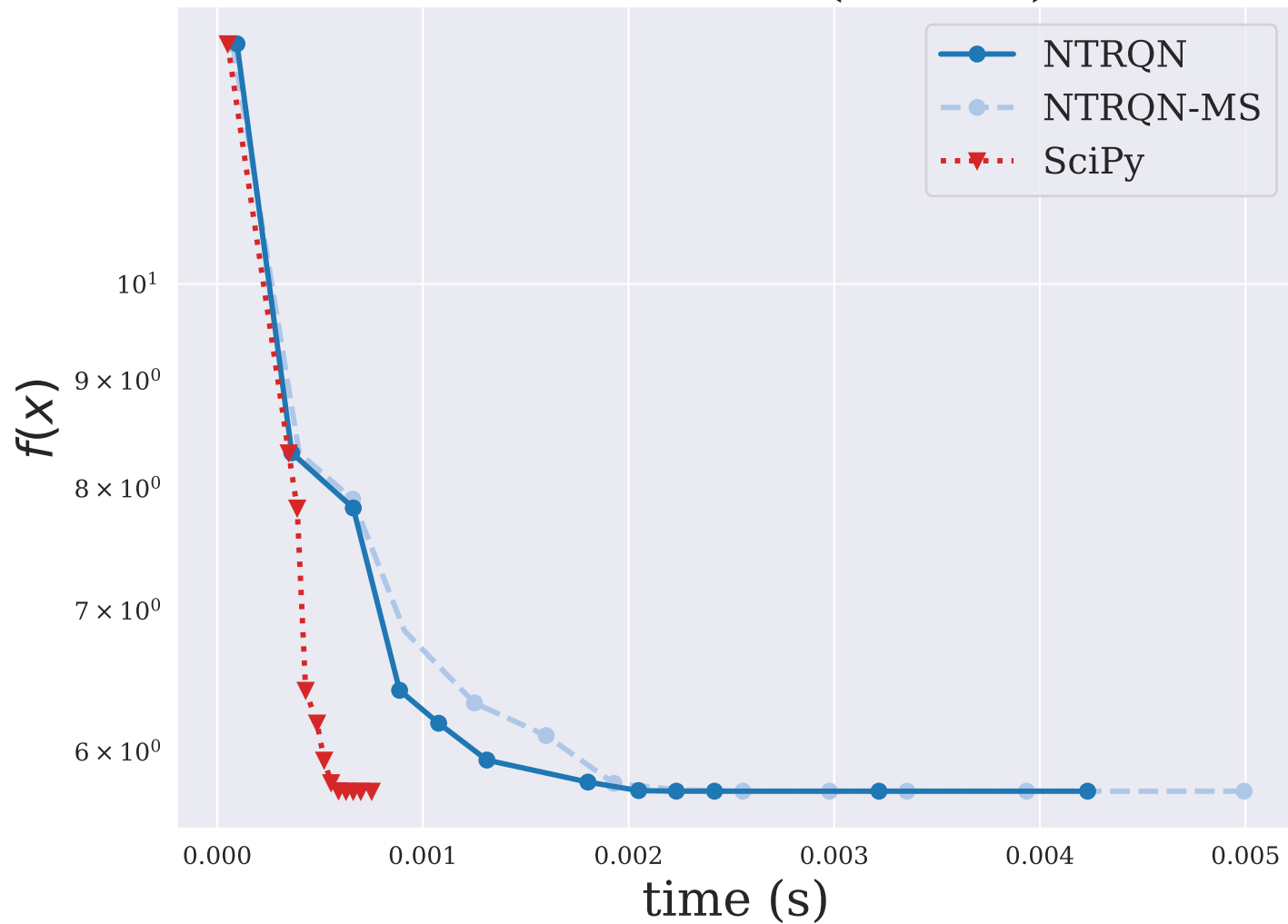
ALLINITU ( n = 4 )
