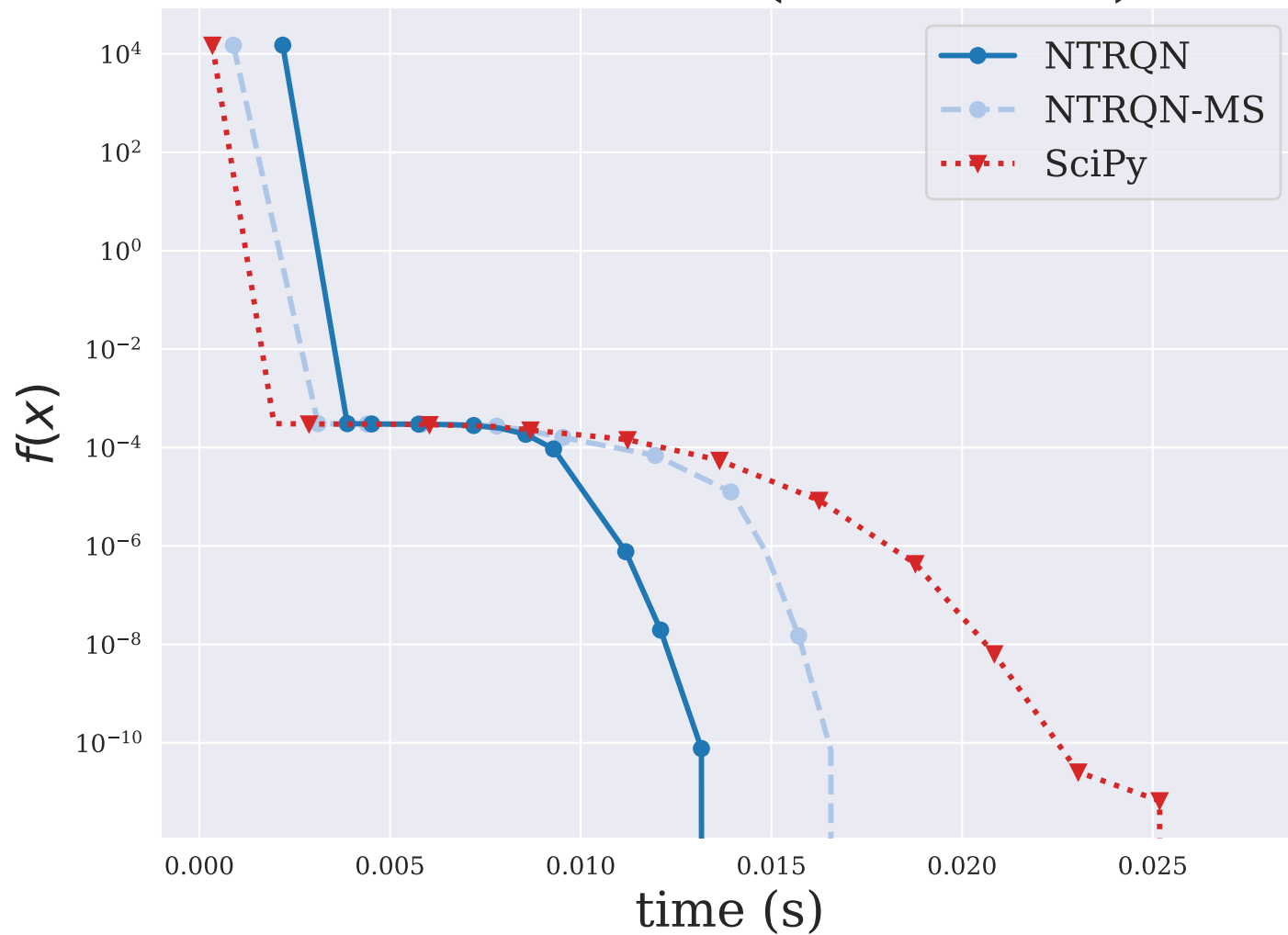
ARWHEAD ( n = 5000 )
