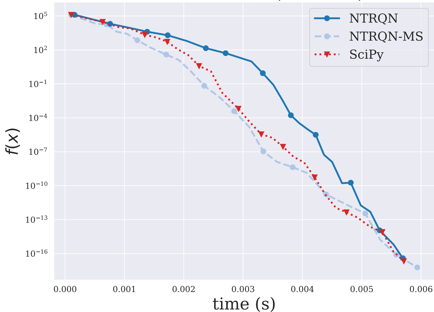
BA-L1SPLS ( n = 57 )
