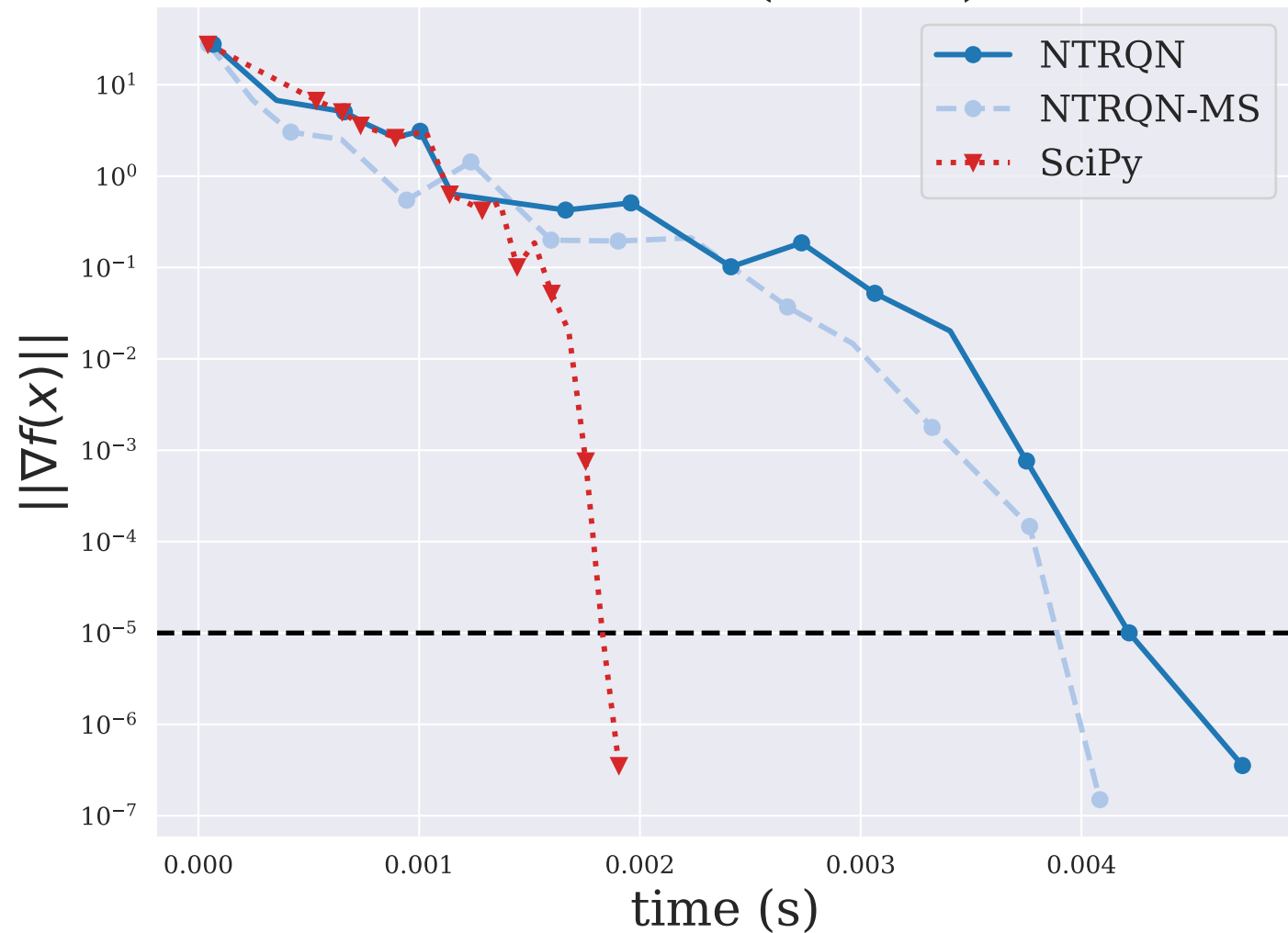
BEALE ( n = 2 )
