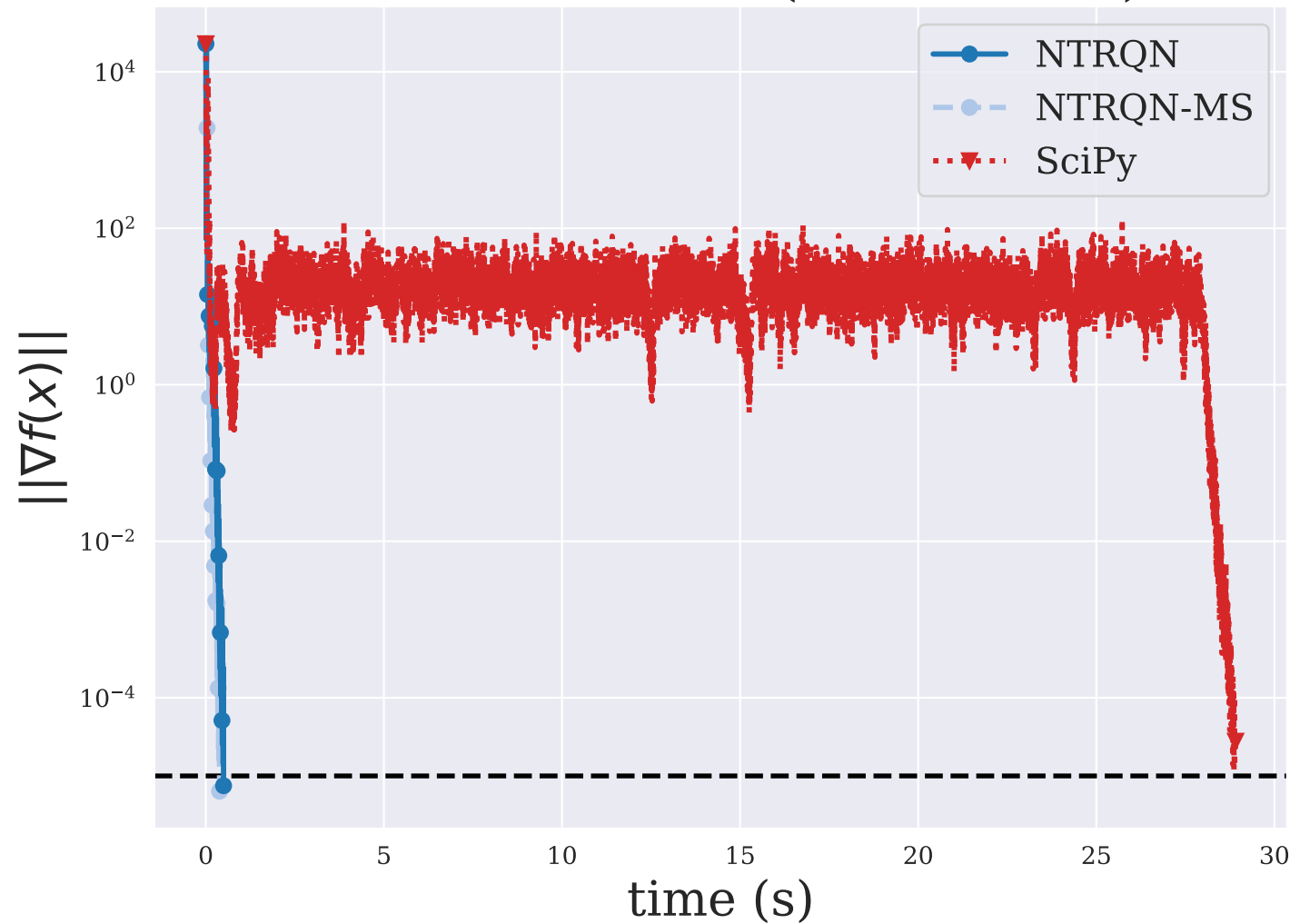
CHAINWOO ( n = 4000 )
