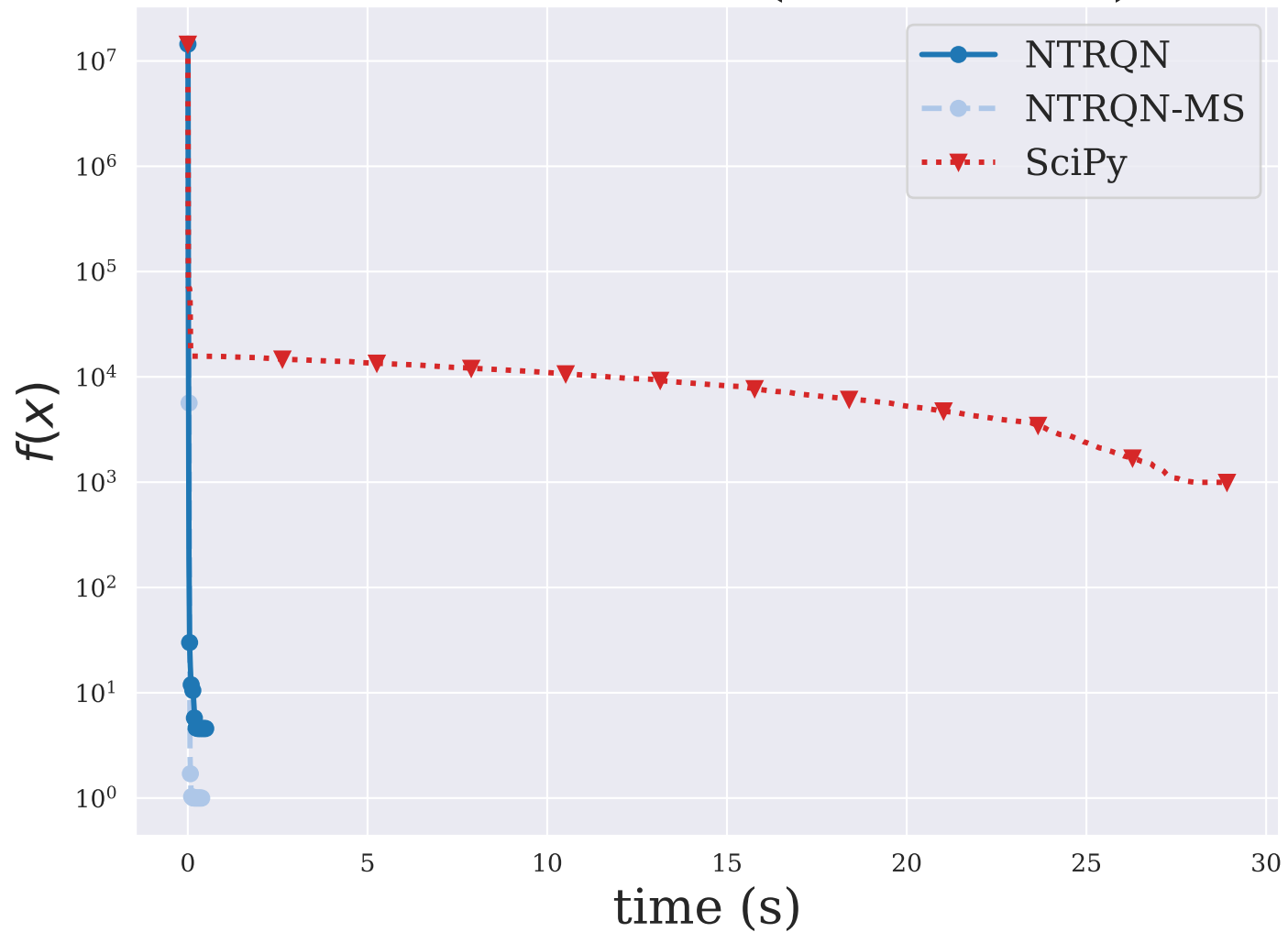
CHAINWOO ( n = 4000 )
