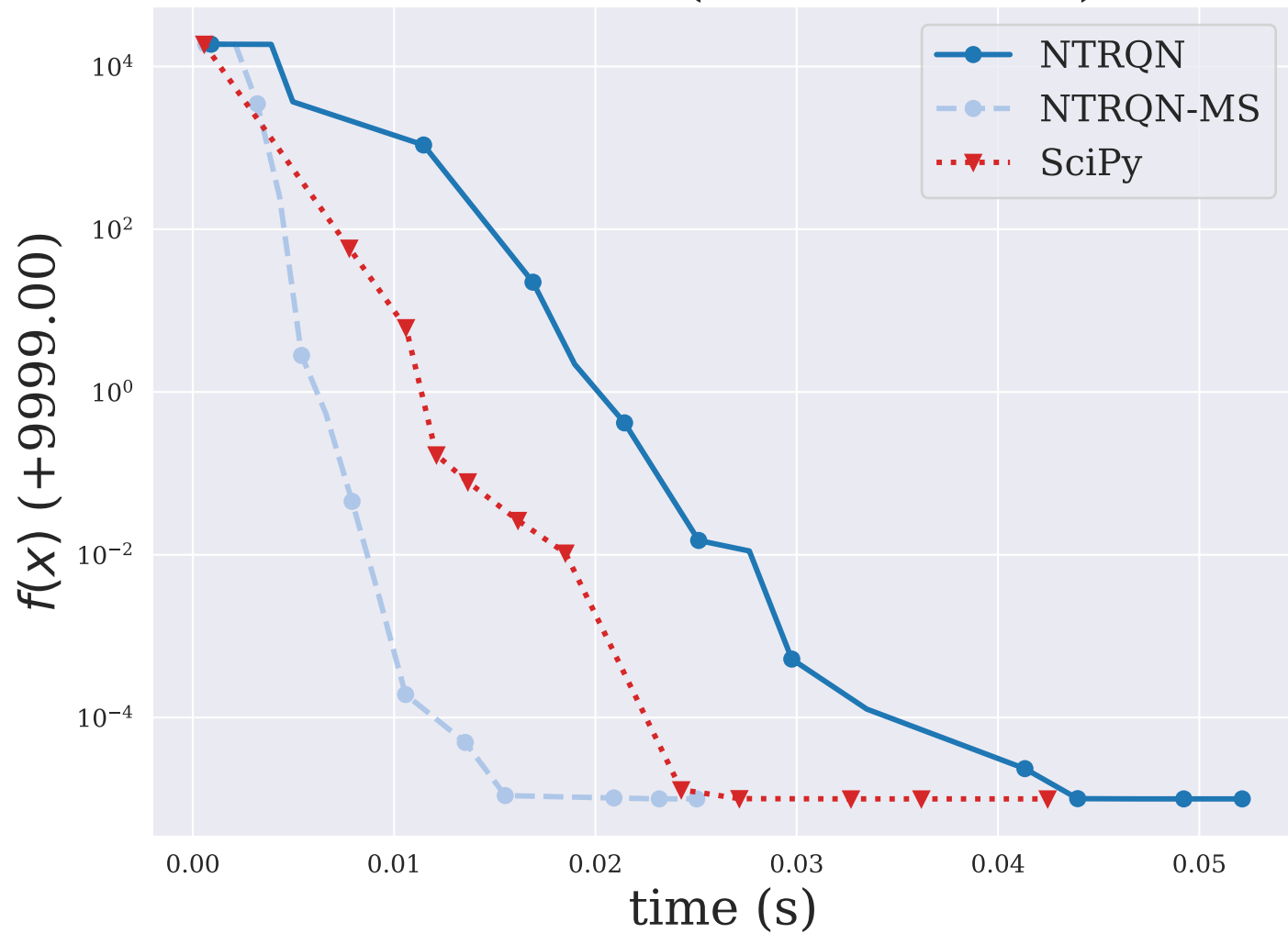
COSINE ( n = 10000 )
