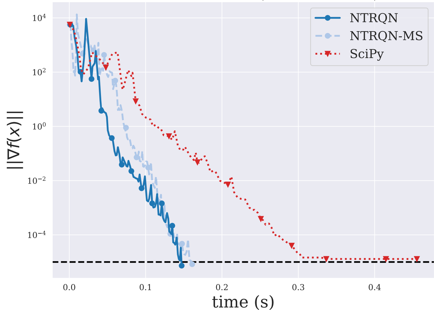
CRAGGLVY ( n = 5000 )
