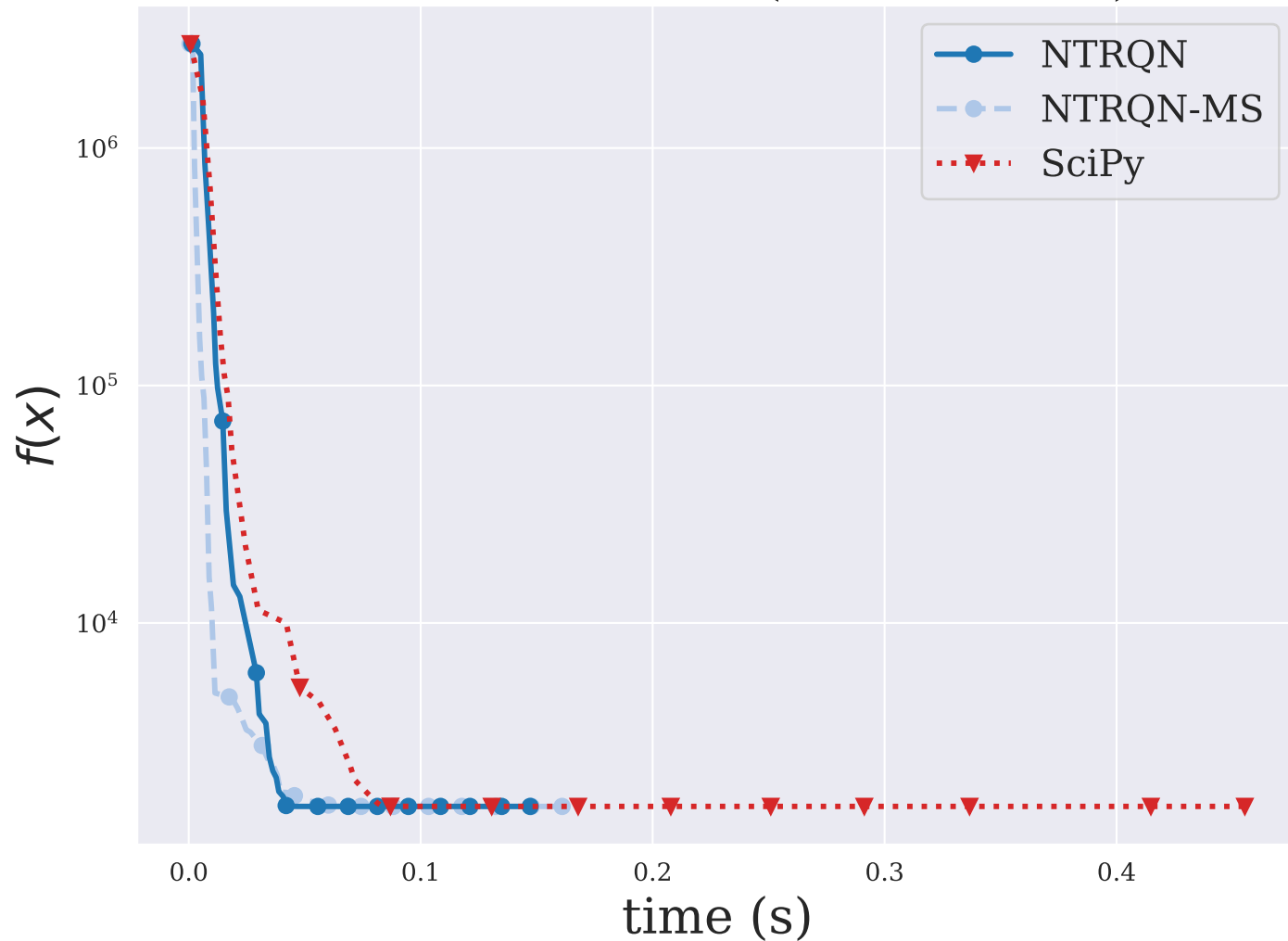
CRAGGLVY ( n = 5000 )
