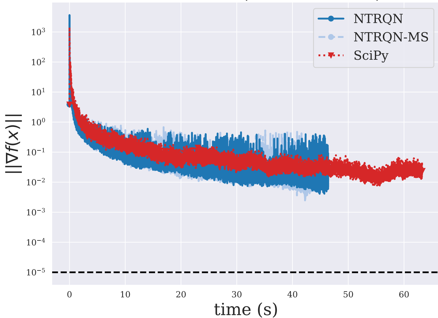
CURLY20 ( n = 10000 )
