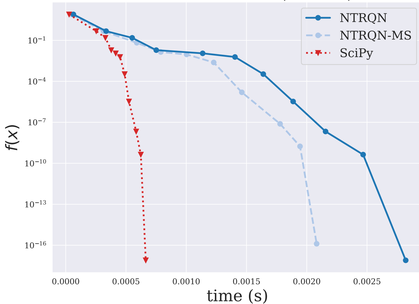
DENSCHNA ( n = 2 )
