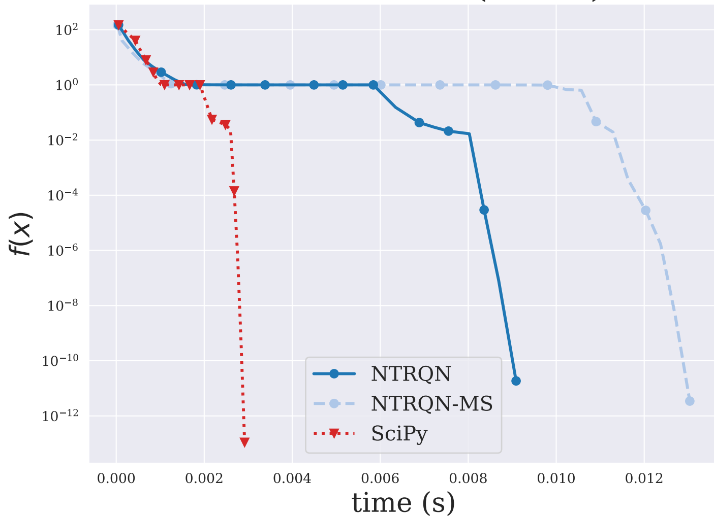
DENSCHNE ( n = 3 )
