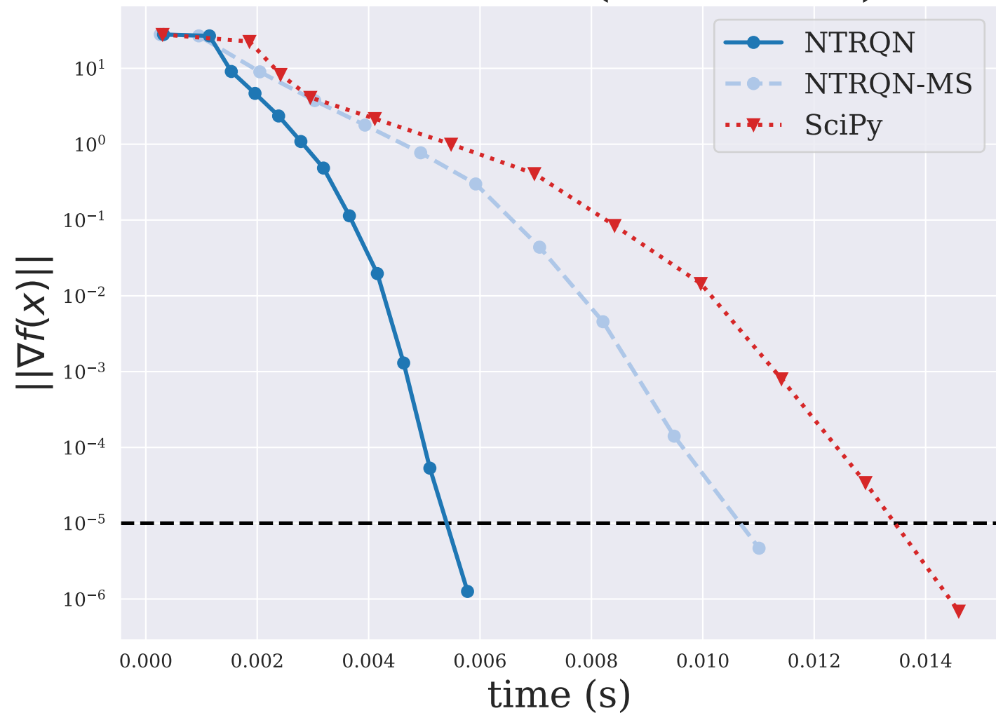
DIXMAANA ( n = 3000 )
