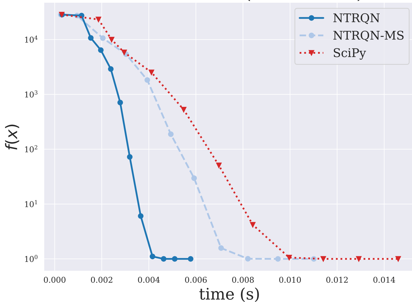
DIXMAANA ( n = 3000 )
