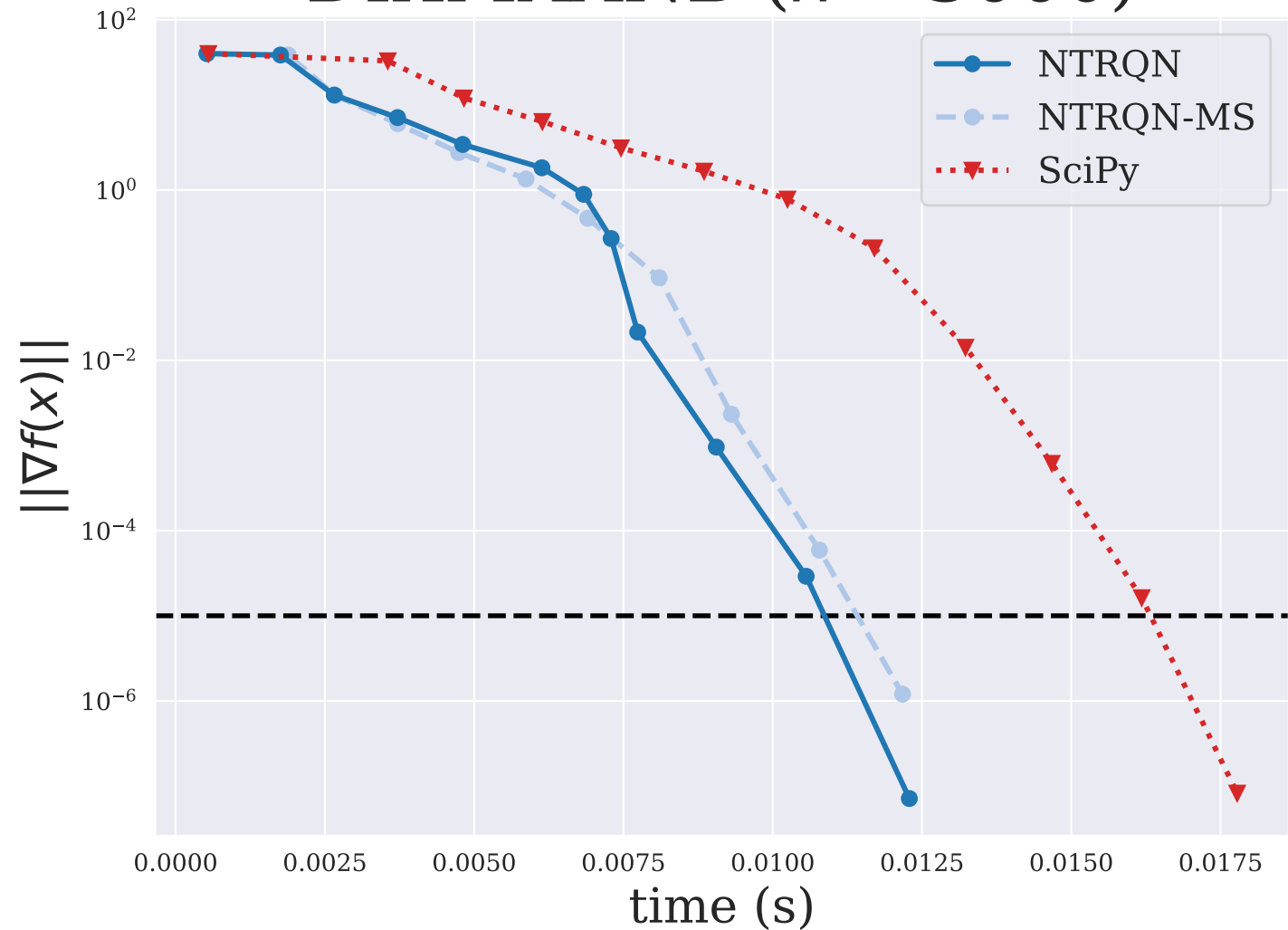
DIXMAANB ( n = 3000 )
