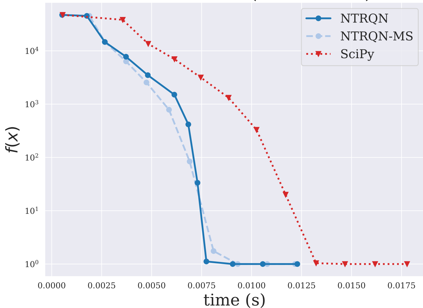
DIXMAANB ( n = 3000 )
