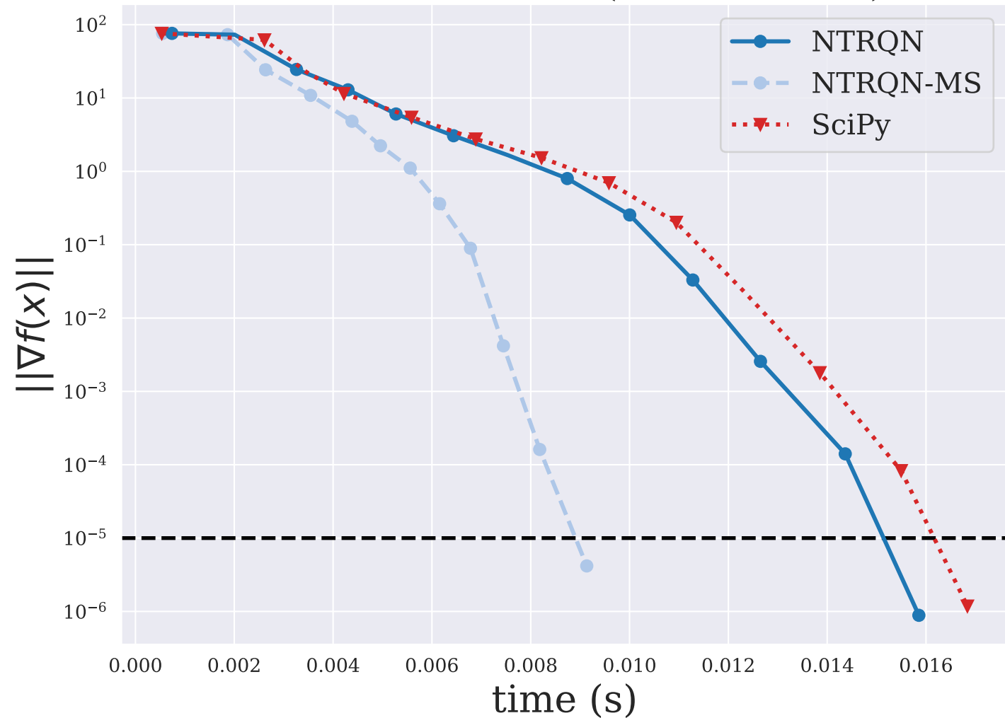
DIXMAANC ( n = 3000 )
