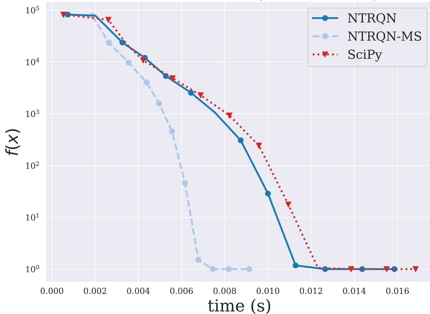
DIXMAANC ( n = 3000 )
