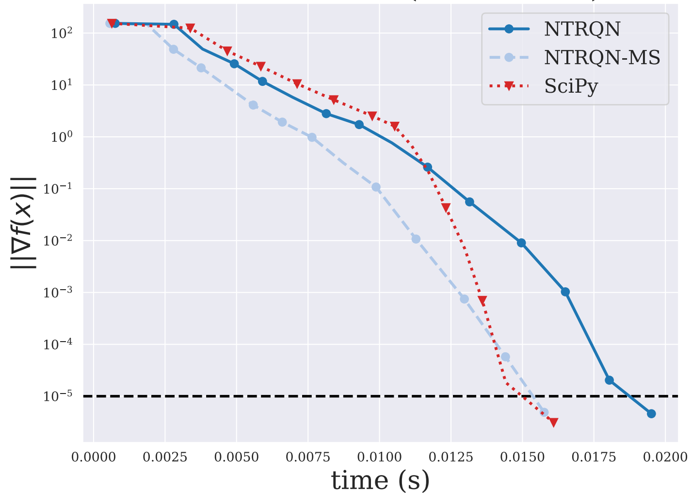
DIXMAAND ( n = 3000 )
