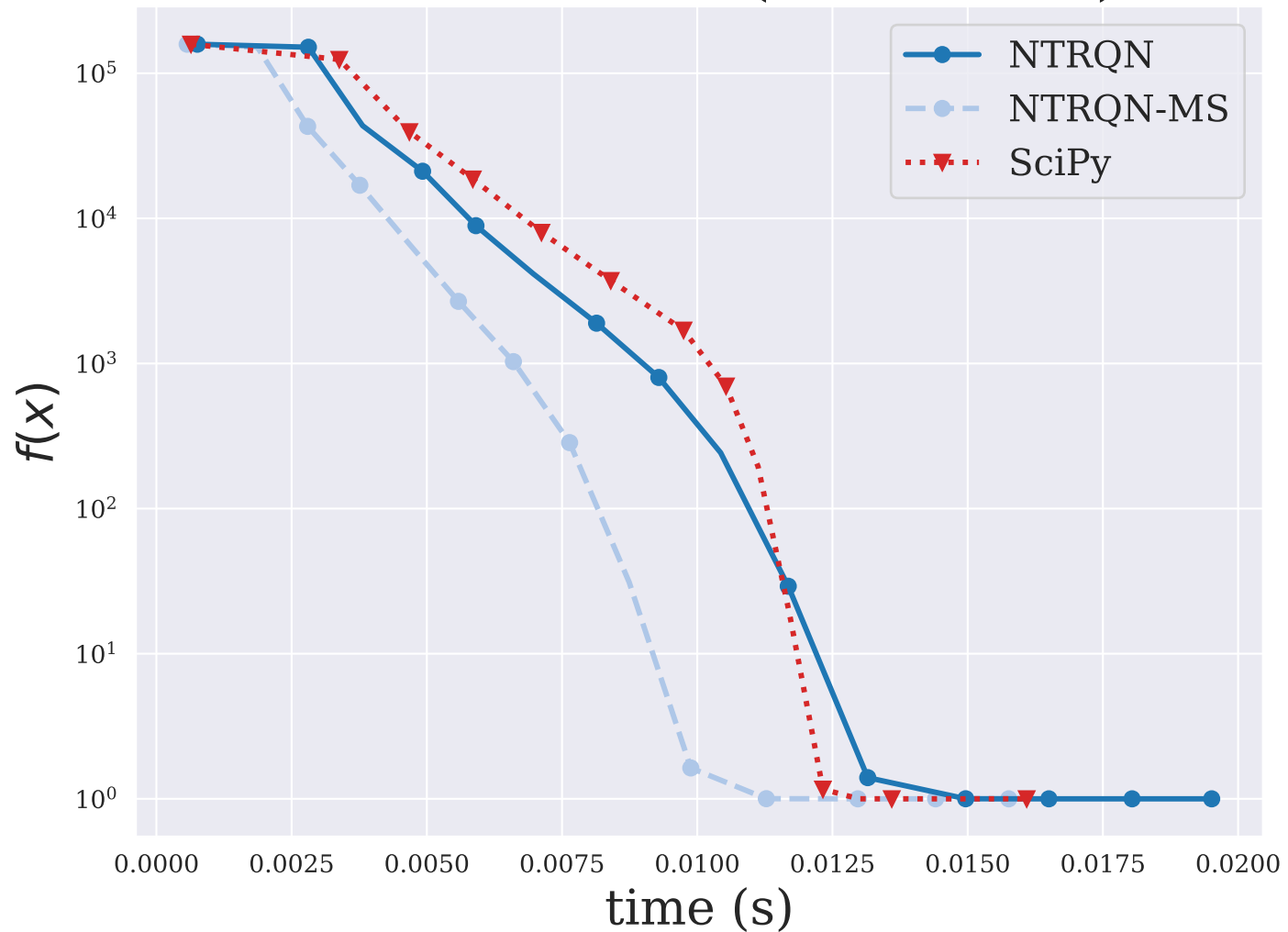
DIXMAAND ( n = 3000 )
