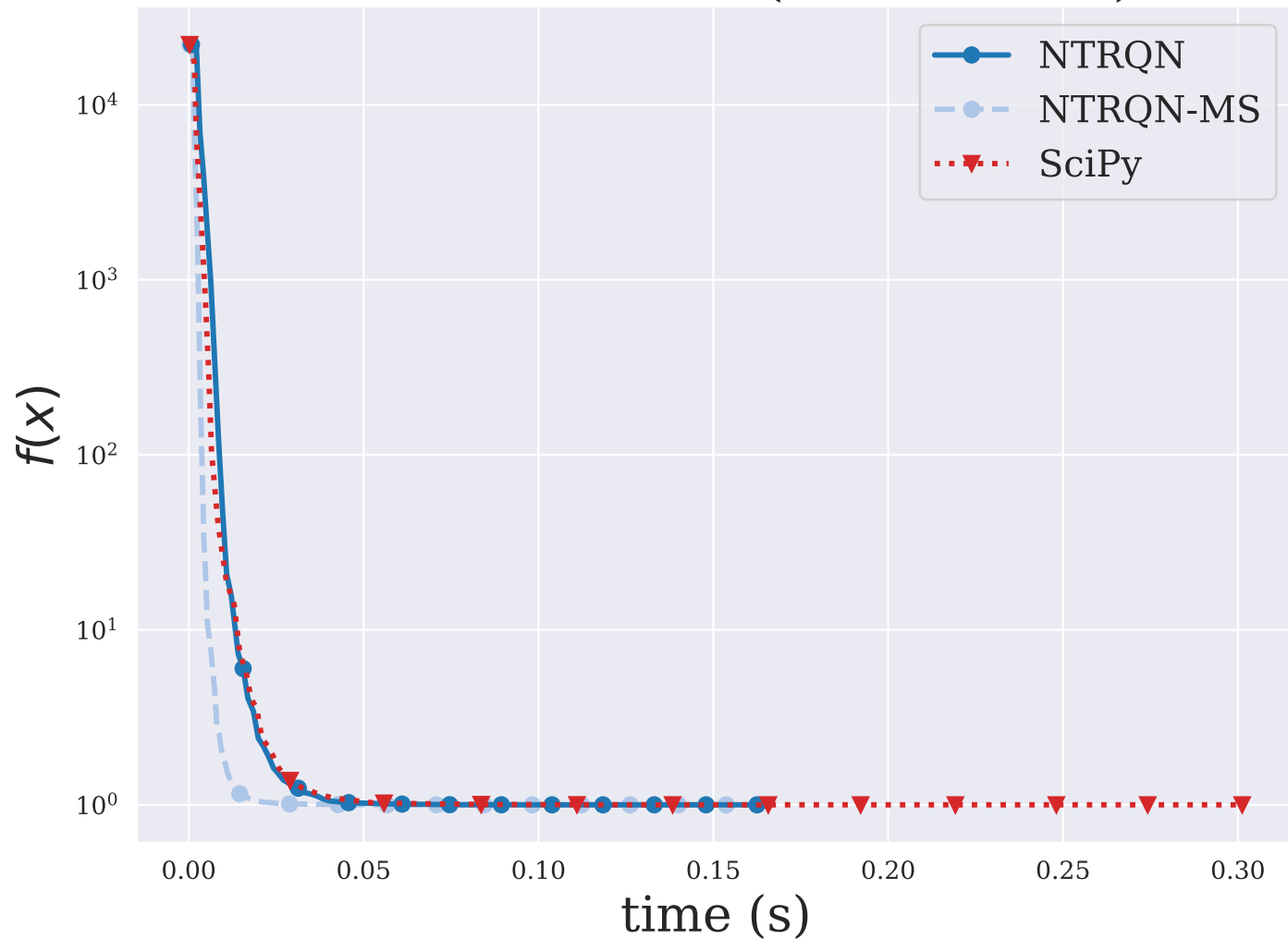
DIXMAANE ( n = 3000 )
