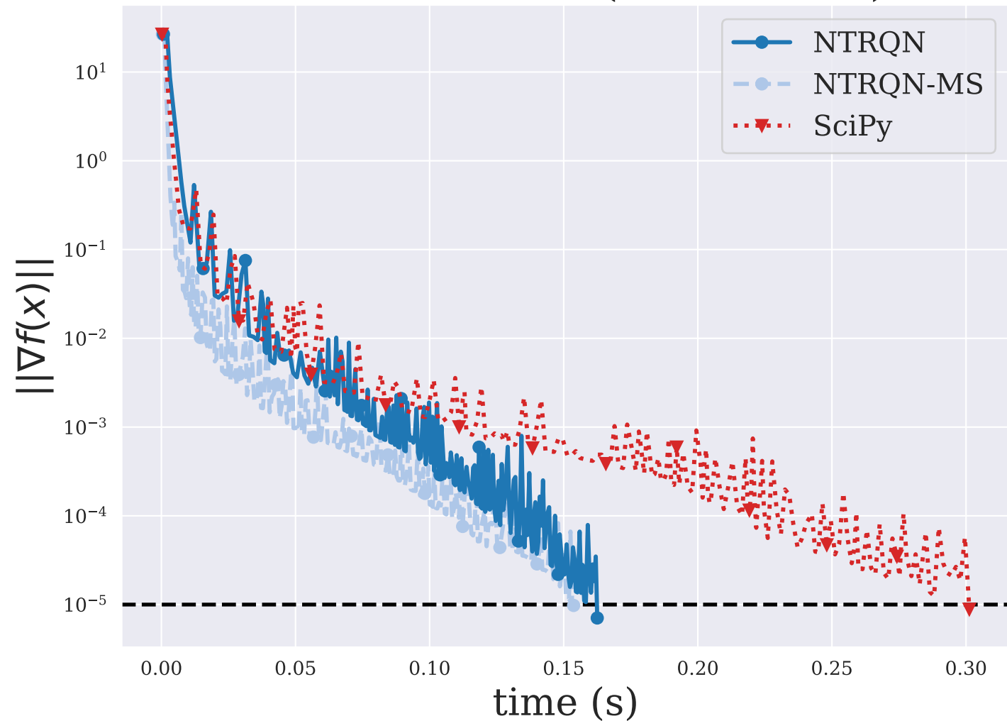
DIXMAANE ( n = 3000 )
