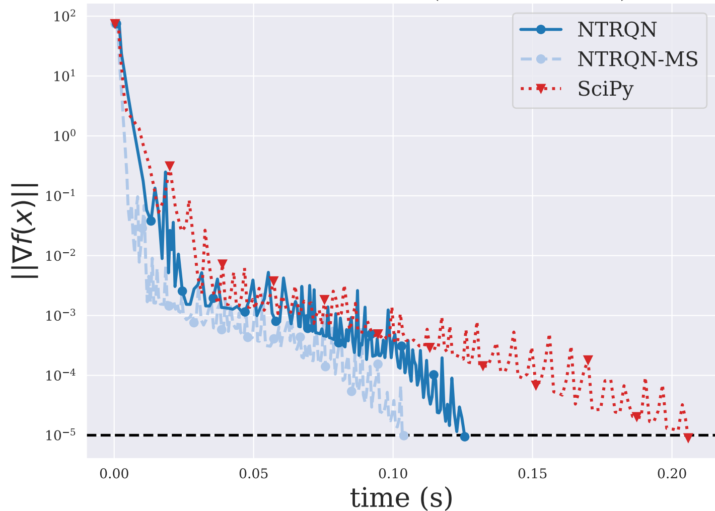
DIXMAANG ( n = 3000 )
