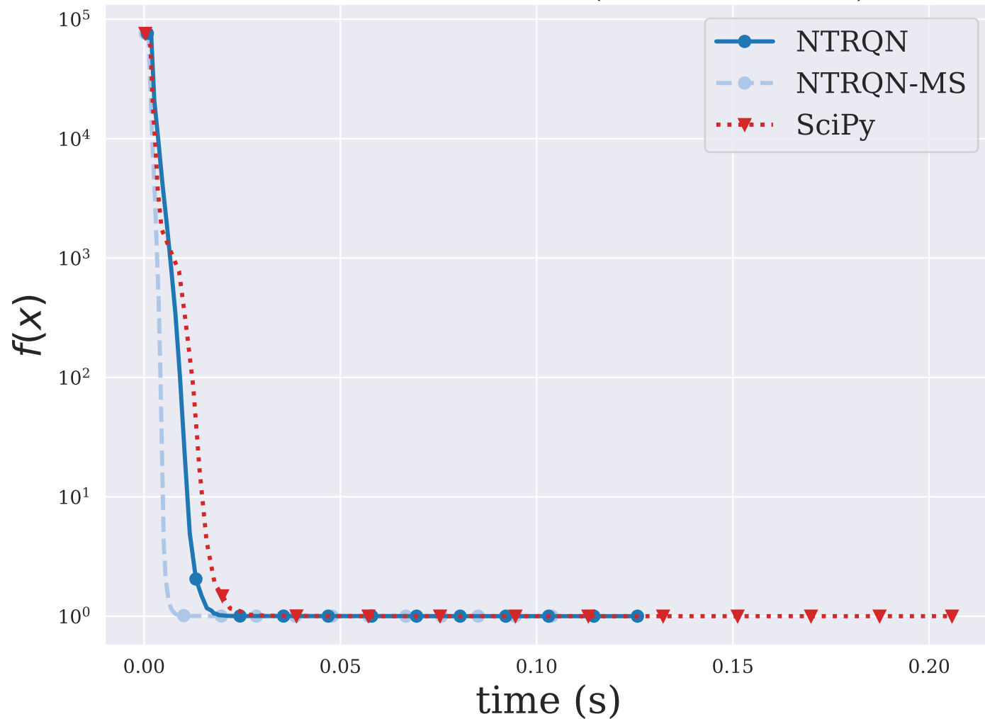
DIXMAANG ( n = 3000 )
