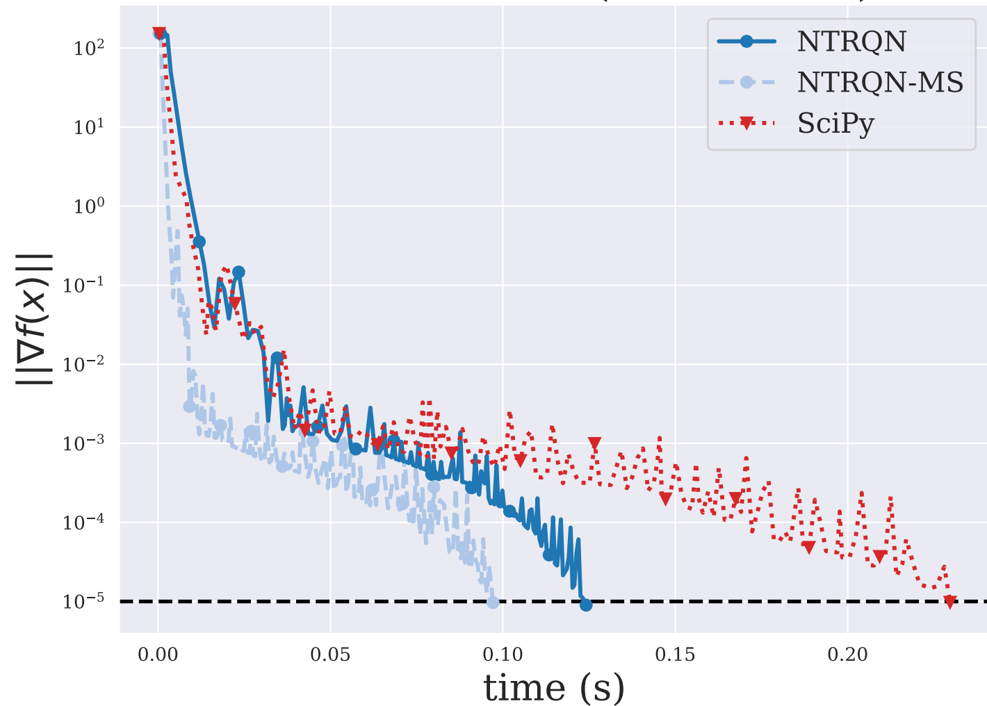
DIXMAANH ( n = 3000 )
