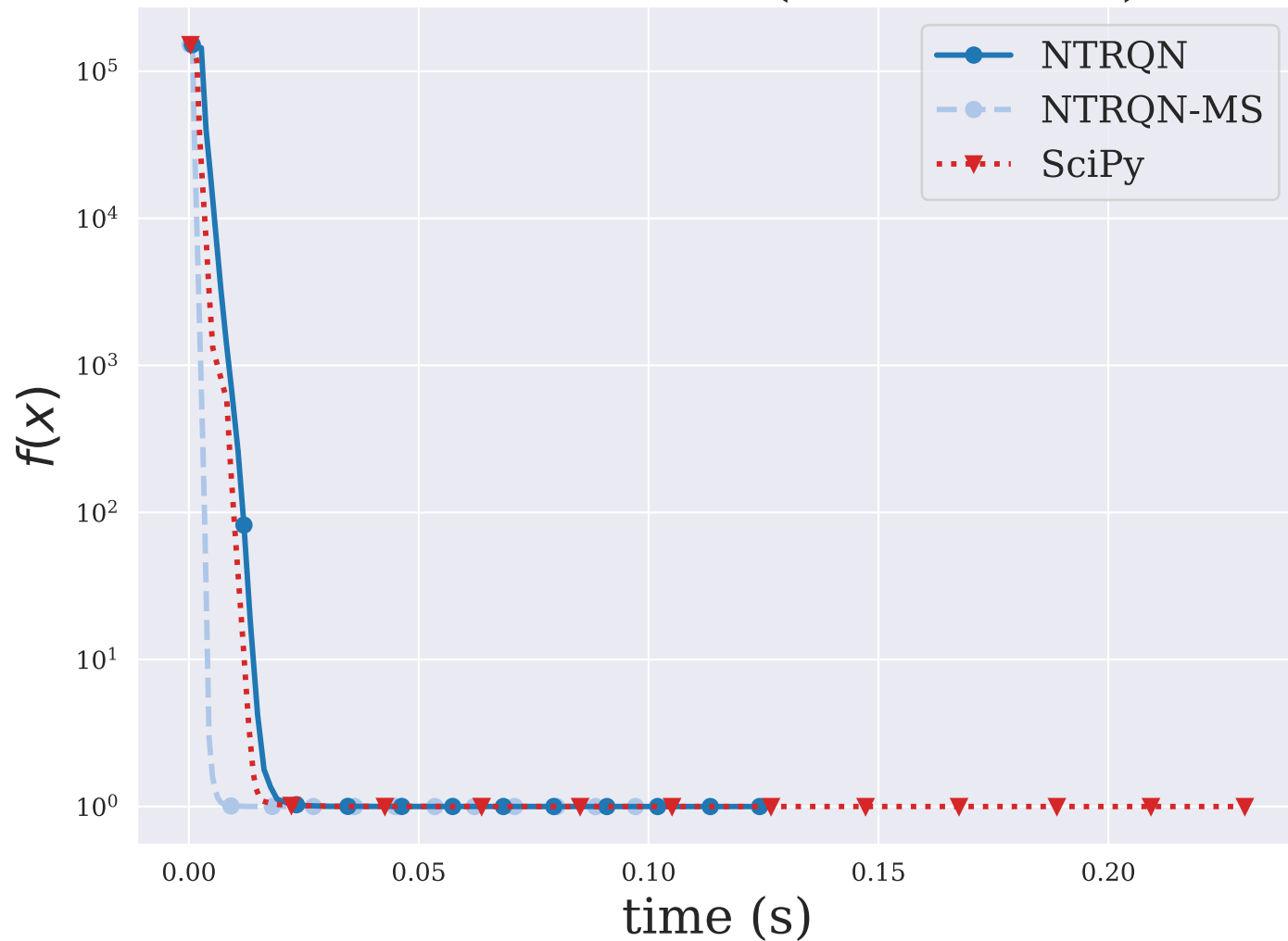
DIXMAANH ( n = 3000 )
