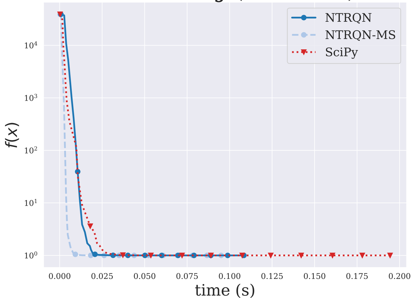
DIXMAANJ ( n = 3000 )
