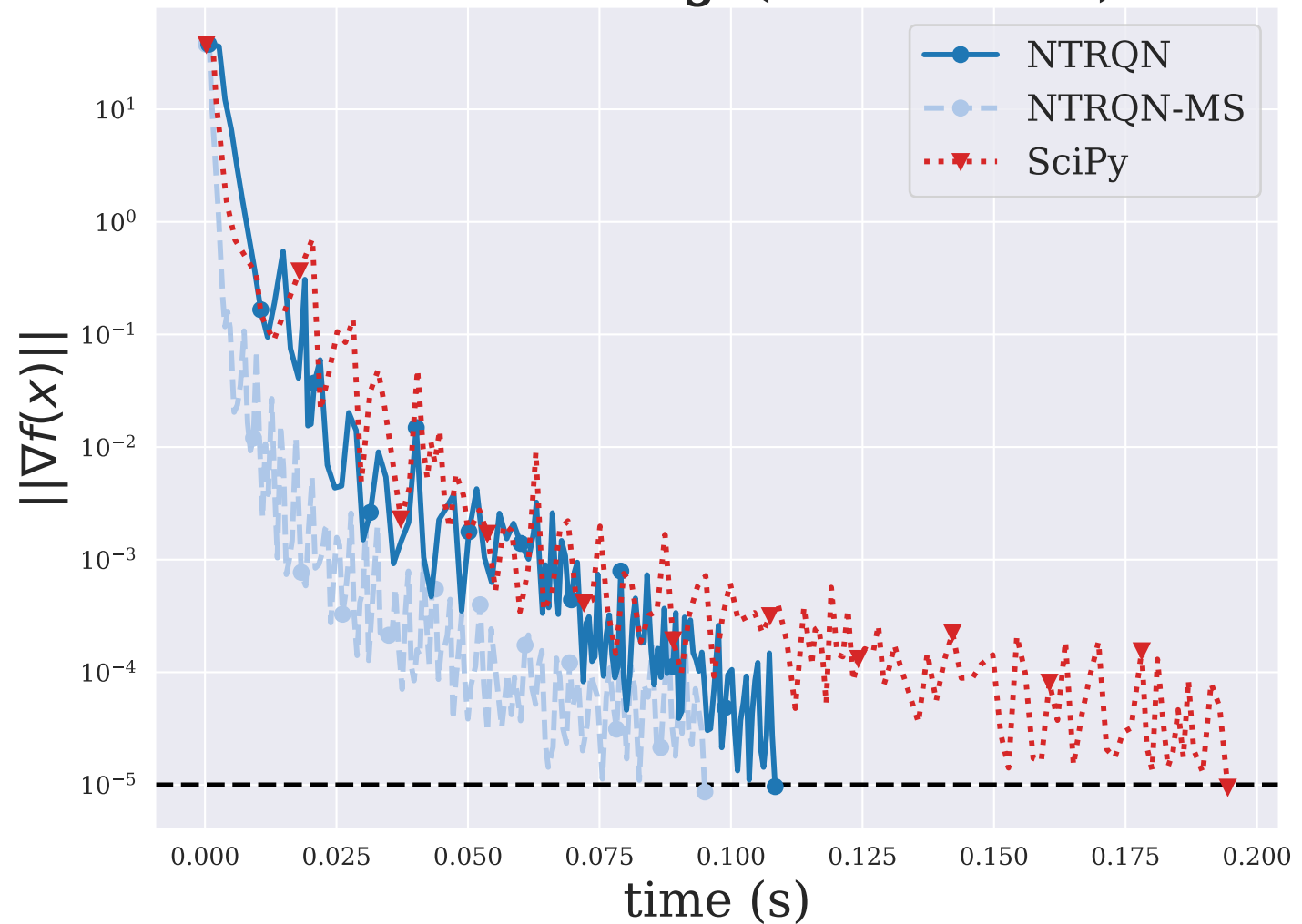
DIXMAANJ ( n = 3000 )
