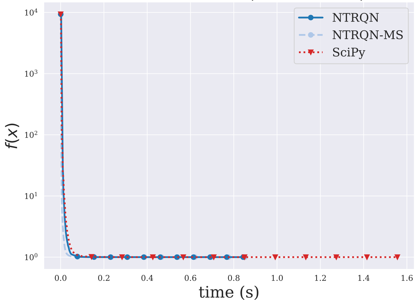
DIXMAANM ( n = 3000 )
