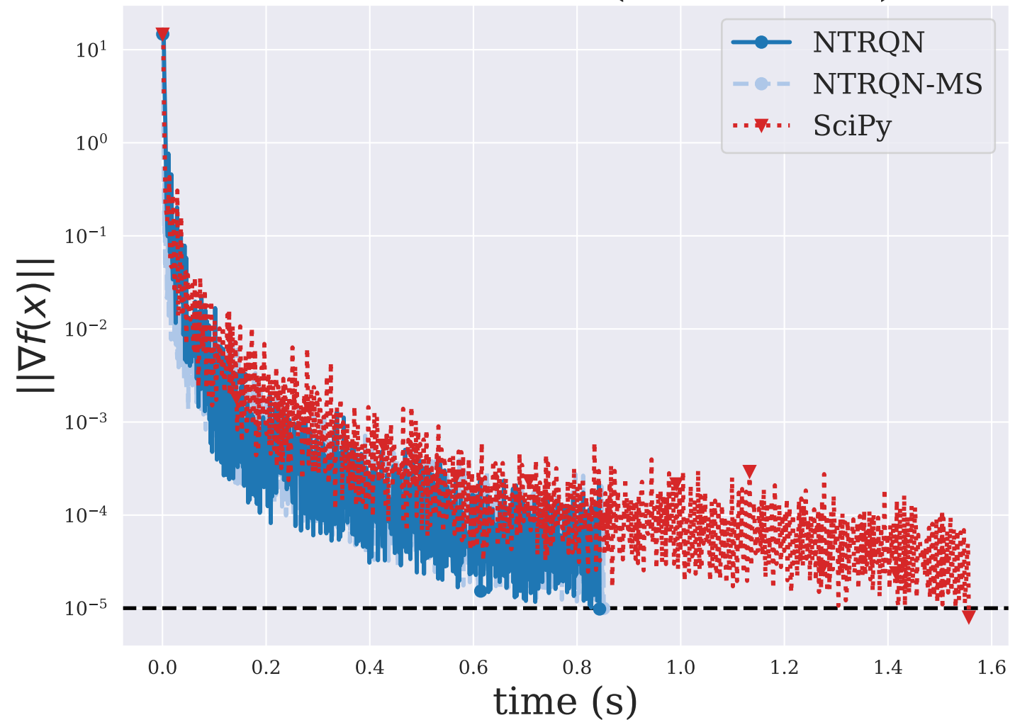
DIXMAANM ( n = 3000 )
