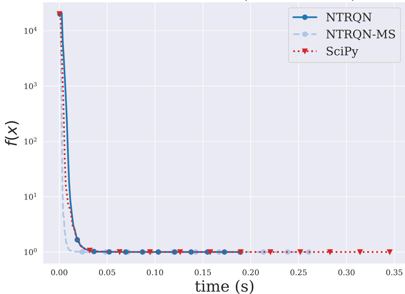
DIXMAANN ( n = 3000 )
