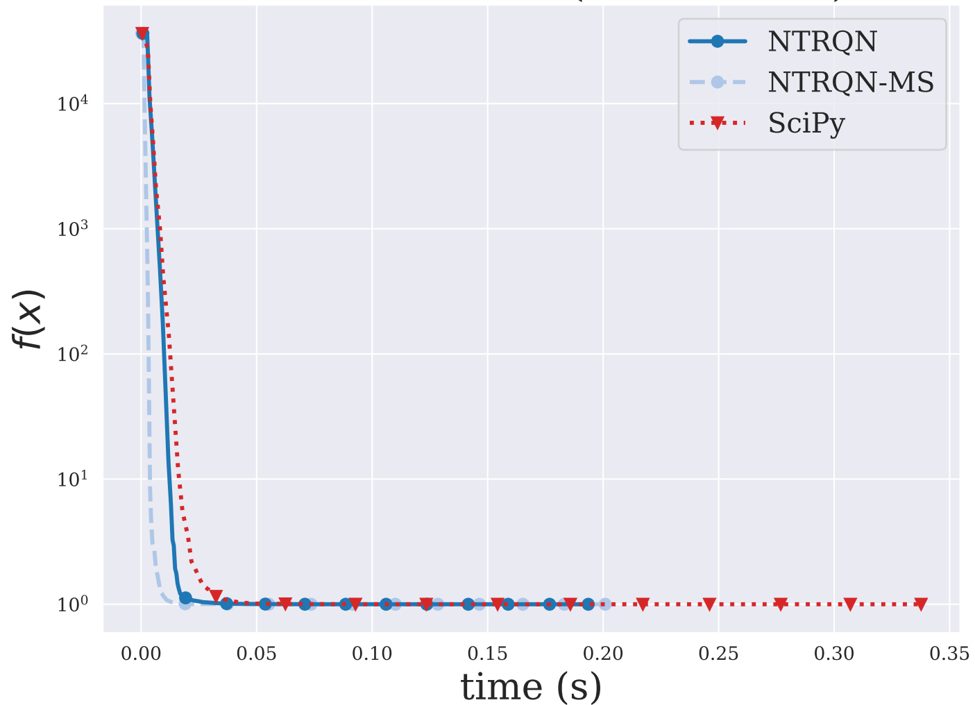
DIXMAANO ( n = 3000 )
