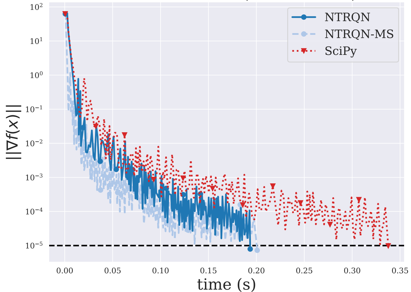
DIXMAANO ( n = 3000 )
