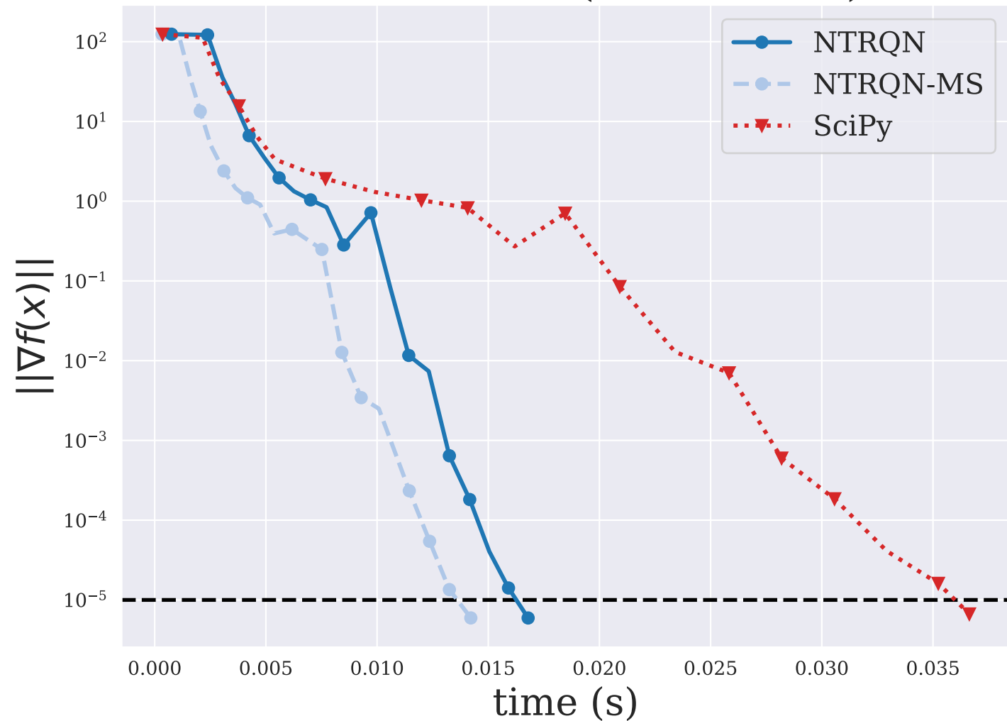
ENGVAL1 ( n = 5000 )
