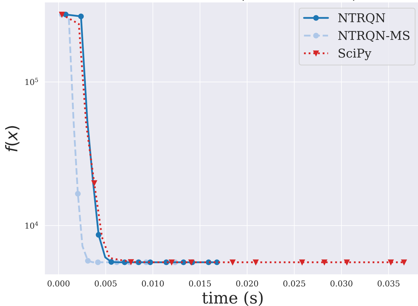
ENGVAL1 ( n = 5000 )
