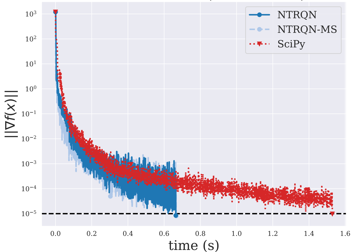
EXTROSNB ( n = 1000 )
