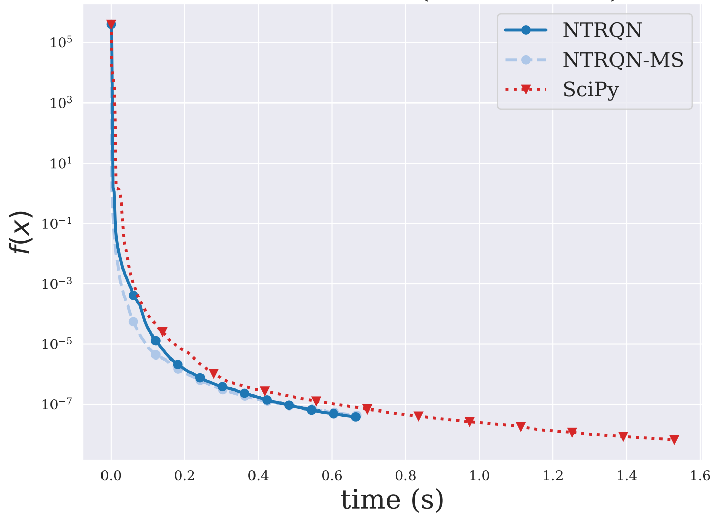
EXTROSNB ( n = 1000 )
