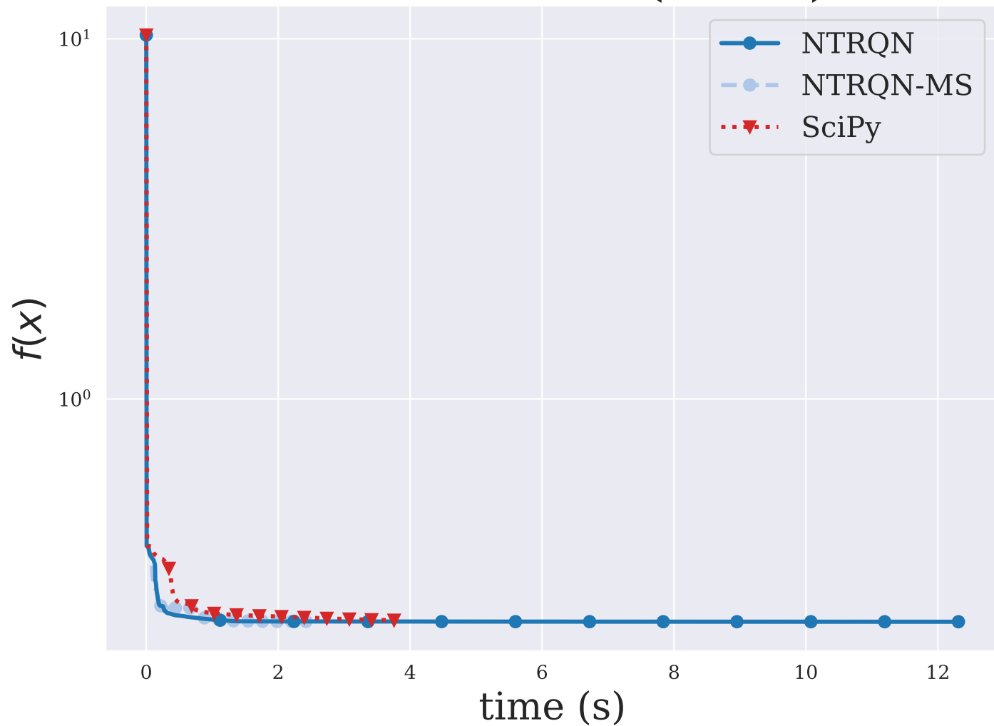
FBRAIN3LS ( n = 6 )
