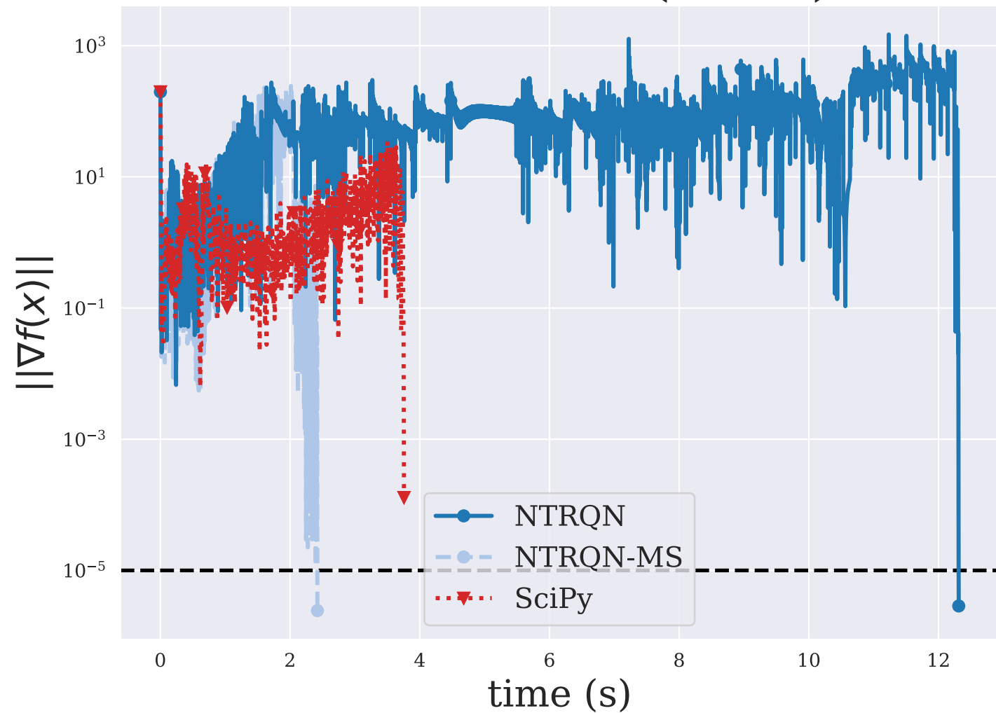
FBRAIN3LS ( n = 6 )
