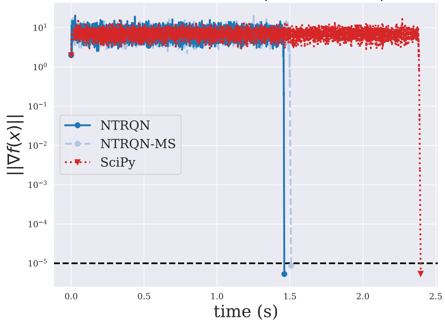
FLETCHCR ( n = 1000 )
