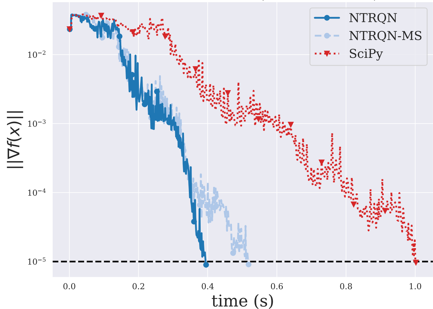
FMINSURF ( n = 5625 )
