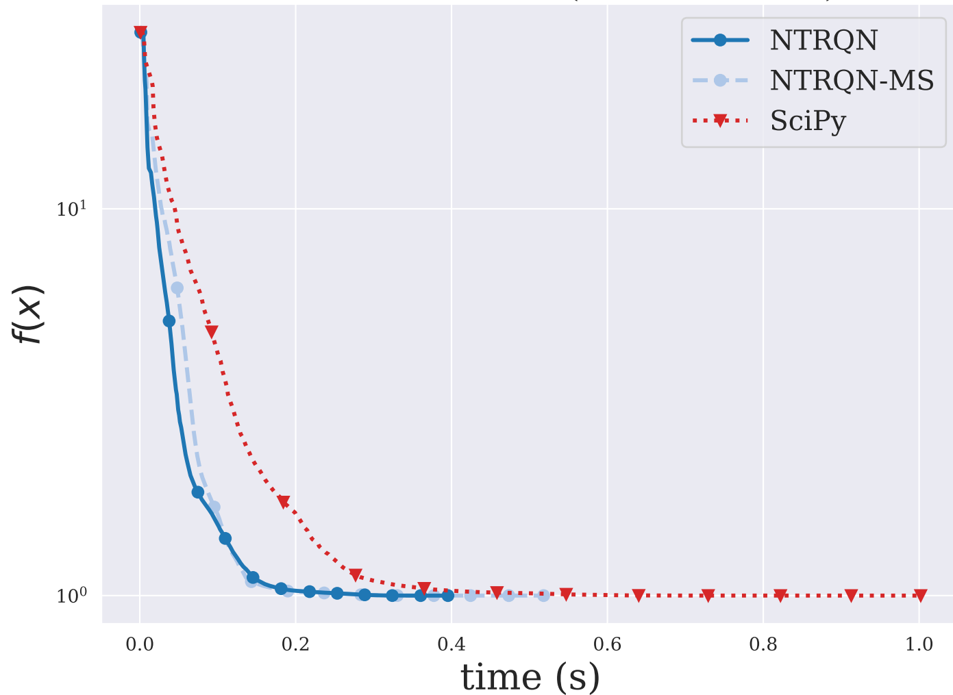
FMINSURF ( n = 5625 )
