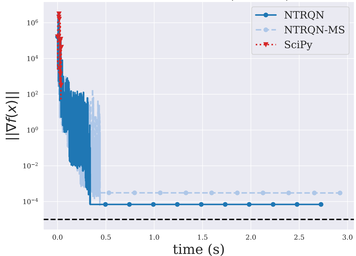
GAUSS1LS ( n = 8 )
