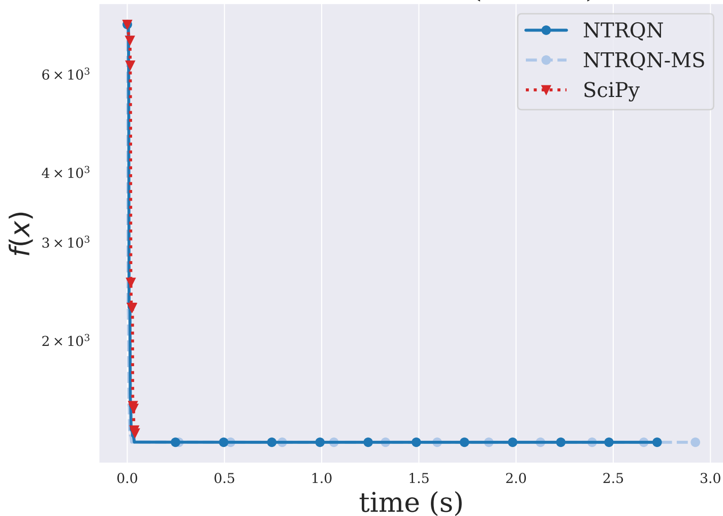
GAUSS1LS ( n = 8 )
