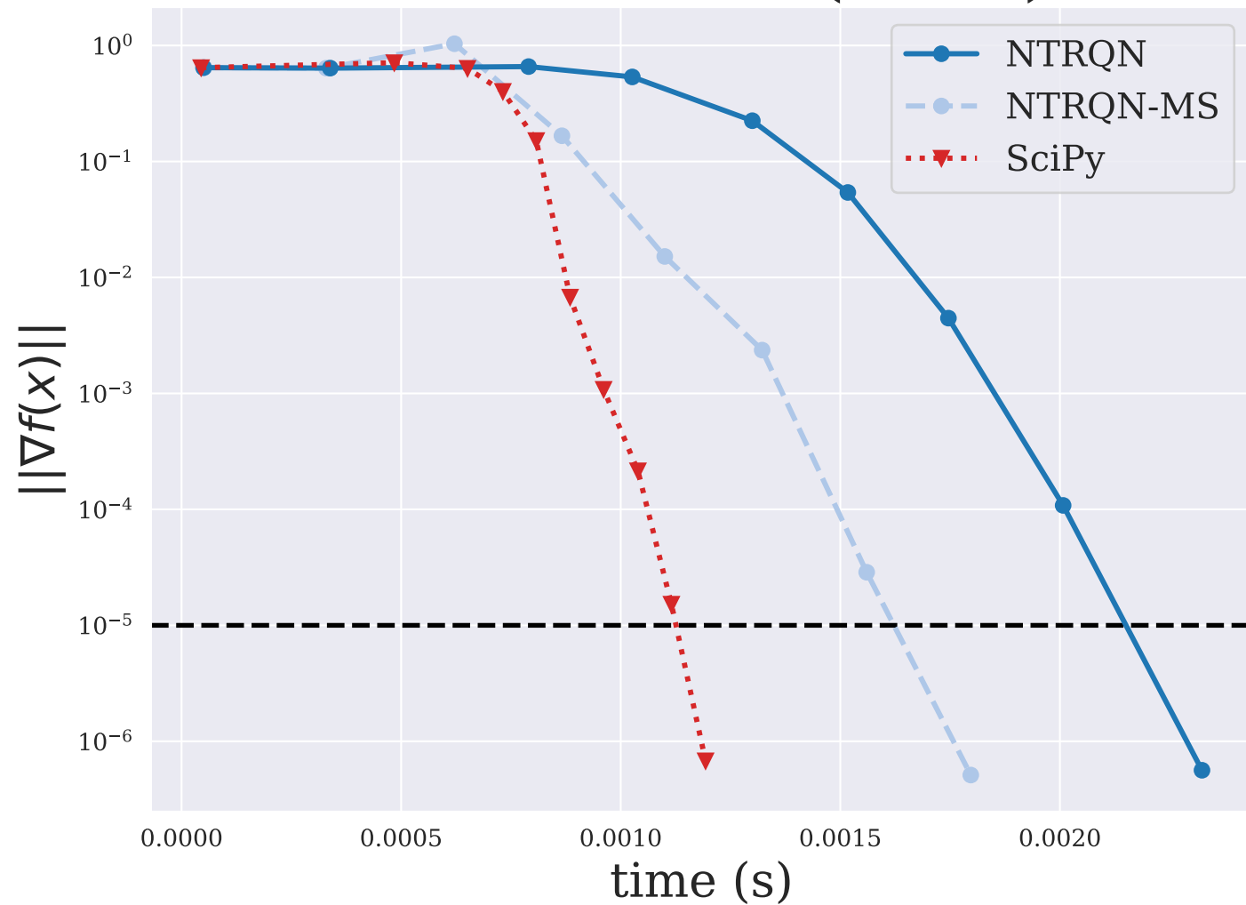
HIMMELBG ( n = 2 )
