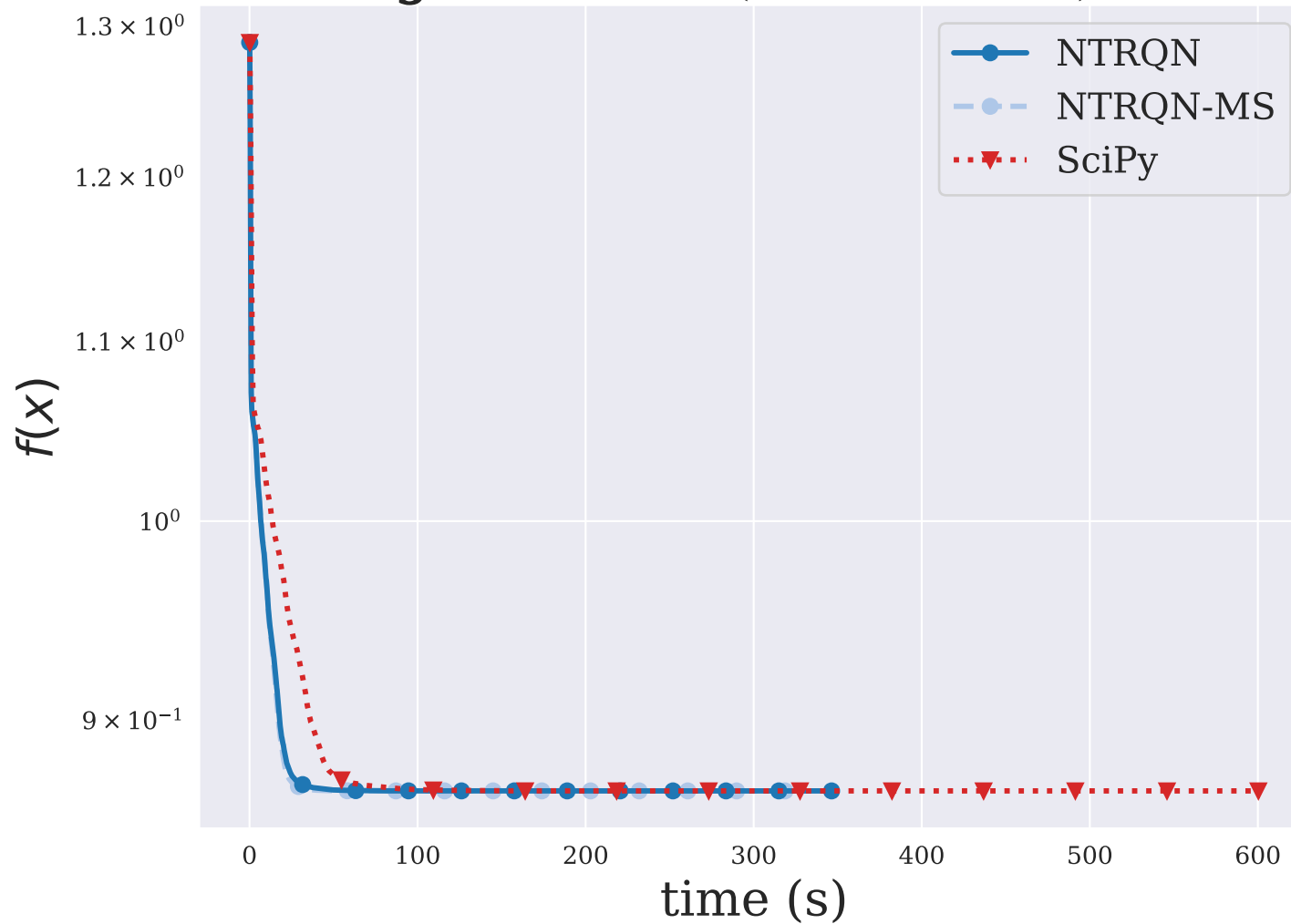
JIMACK ( n = 3549 )
