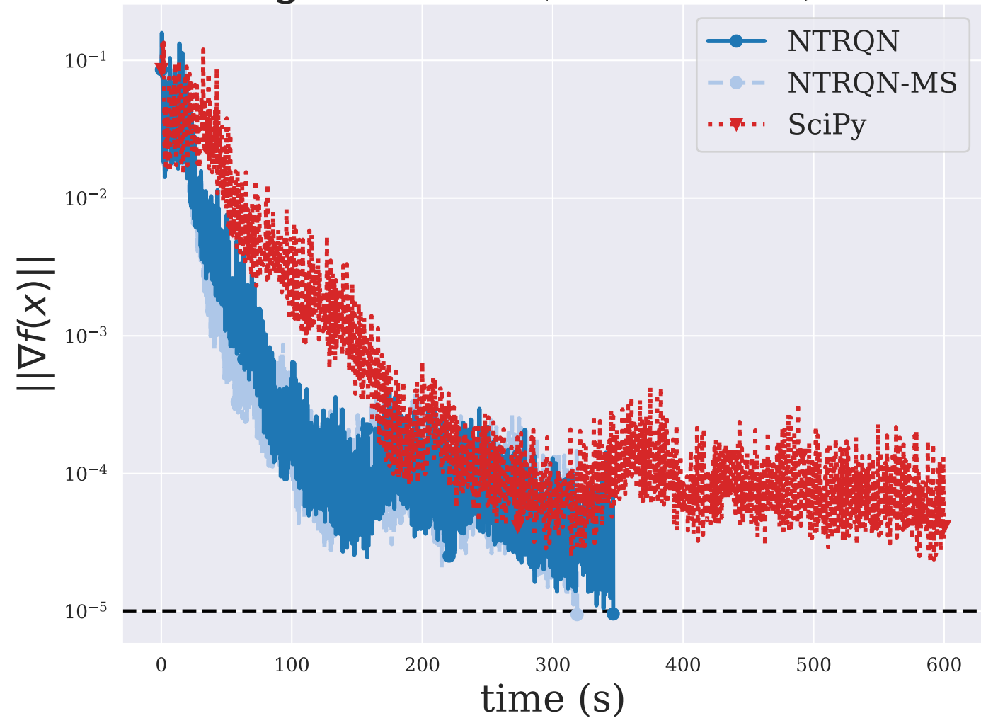
JIMACK ( n = 3549 )
